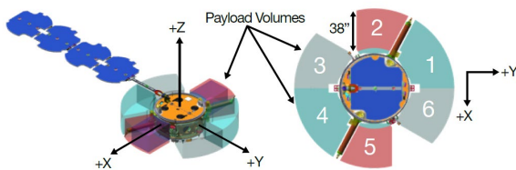
Figure 3: LDPE accommodation wedges establishing virtual canister boundaries
