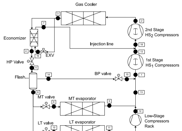
Figure 6: SCVI Layout
