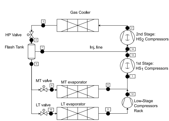
Figure 5: FTVI Layout
