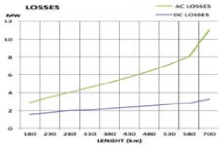
(a) Losses in AC and DC Lines
