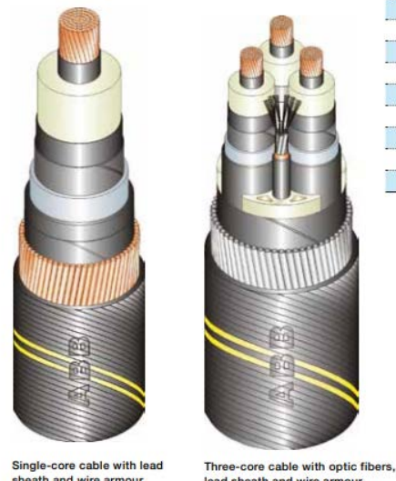
Figure 6: Physical Cable View, HVAC vs HVDC
