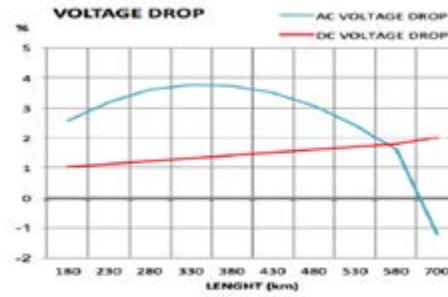
(b) Voltage Drop Across AC and DC Lines
