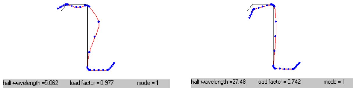
(a) local buckling
