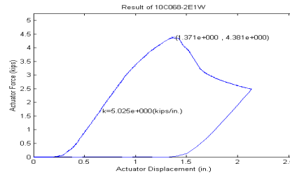
(b) h=10 in. ( M_{test}/M_y=0.6 )
