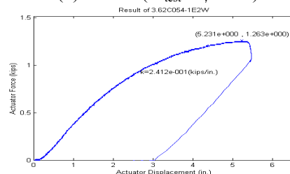
(f) h=3.62 in. ( M_{test}/M_y=1.16 )
