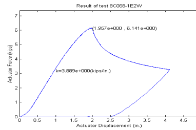
(b) t=0.068 in. ( M_{test}/M_y=0.91 )
