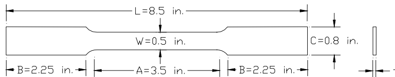
Figure 15 Dimensions of tensile coupon
