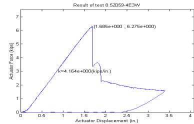
(f) t=0.059 in. ( M_{test}/M_y=0.79 )
