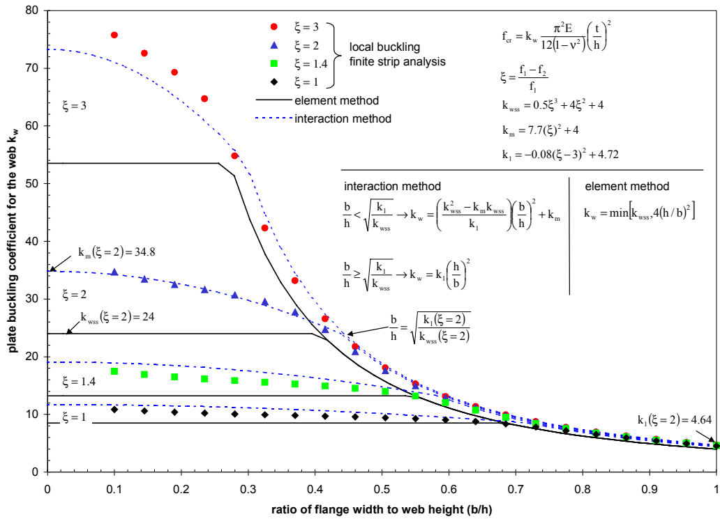
Figure 1 Web plate buckling coefficient as a function of flange width to web height ratio for local buckling including web/flange interaction, approximate hand expressions also given
