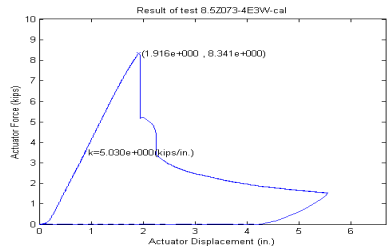
(e) t=0.073 in. ( M_{test}/M_y=0.86 )
