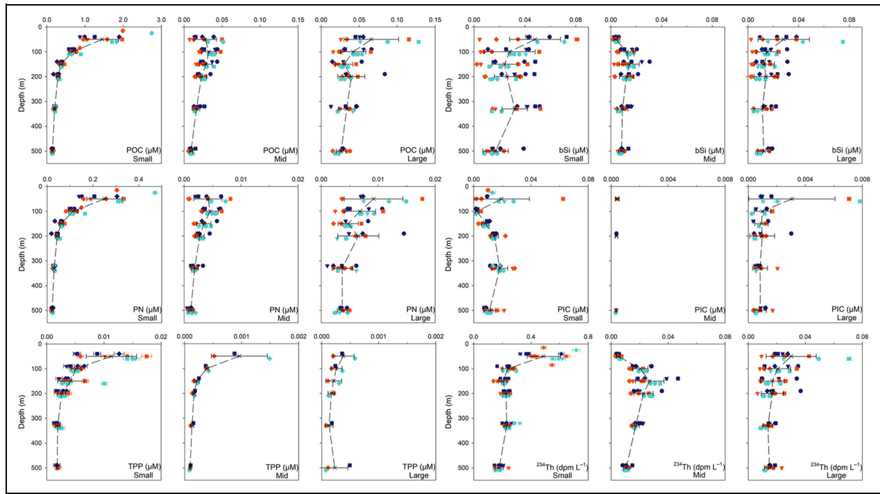
Figure 2. Size-fractionated concentrations of bioelements and thorium-234 ( ^{234}\text{Th} ) versus depth. Particulate organic carbon (POC), particulate nitrogen (PN), total particulate phosphorus (TPP), biogenic silica (bSi), particulate inorganic carbon (PIC), and ^{234}\text{Th} concentrations versus depth in small (1–5 \mu\text{m} ), mid-sized (5–51 \mu\text{m} ), and large (>51 \mu\text{m} ) particles collected during the EXport Processes in the Ocean from RemoTe Sensing cruise near Station P. Each symbol represents a specific in situ pump cast color-coded by sampling “epoch” (Epoch 1 = dark blue, Epoch 2 = red, and Epoch 3 = turquoise), as in Figure 1 . Data from each epoch are offset by 10 m to facilitate visualization. In most cases, error bars are not visible because they are smaller than the symbols. Error bars were obtained by propagating the standard deviation of the process blanks and other sources of error (see Section 2.3). Black crosses show average ( \pm standard deviation) concentrations at 50, 100, 150, 200, 330, and 500 m. Five additional data points for POC, PN, PIC, and ^{234}\text{Th} in small particles from 20, 85, and 320 m (Epochs 2 and 3) are shown on the left panels. Note different scales on the x-axes between small versus mid-sized and large particles, except for bSi. DOI: https://doi.org/10.1525/elementa.2020.00166.f2
