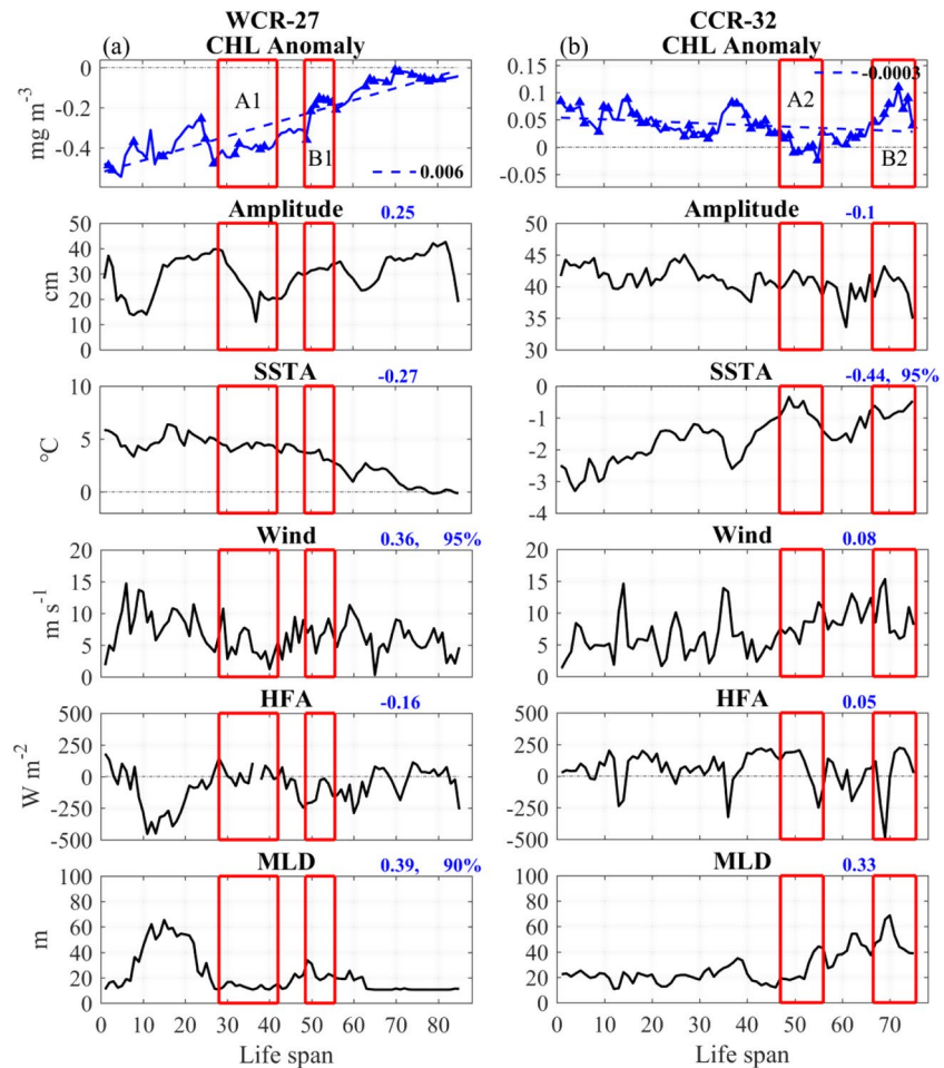
Figure 3. Time series of CHLA, amplitude, SSTA, wind, net heat flux anomaly, and MLD in WCR-27 (a) and CCR-32 (b). The lifespans of WCR-27 and CCR-32 are from April 19, 2012 to July 12, 2012 and from August 17, 2010 to October 30, 2010, respectively. The locations of WCR-27 and CCR-32 where they were first identified are (40.6°N, 61.9°W) and (39.1°N, 56.4°W), respectively. The number on the top of each subpanel represents the correlation coefficient between each variable with CHLA. Significant correlations above 90% level based on t-test are also shown. Blue triangle in the top panel represents the value obtained from level-3 products. Red rectangles highlight two contrasting periods for the WCR and CCR. CCR, cold-core ring; CHLA, chlorophyll anomaly; MLD, mixed layer depth; SSTA, sea surface temperature anomaly; WCR, warm-core ring.
