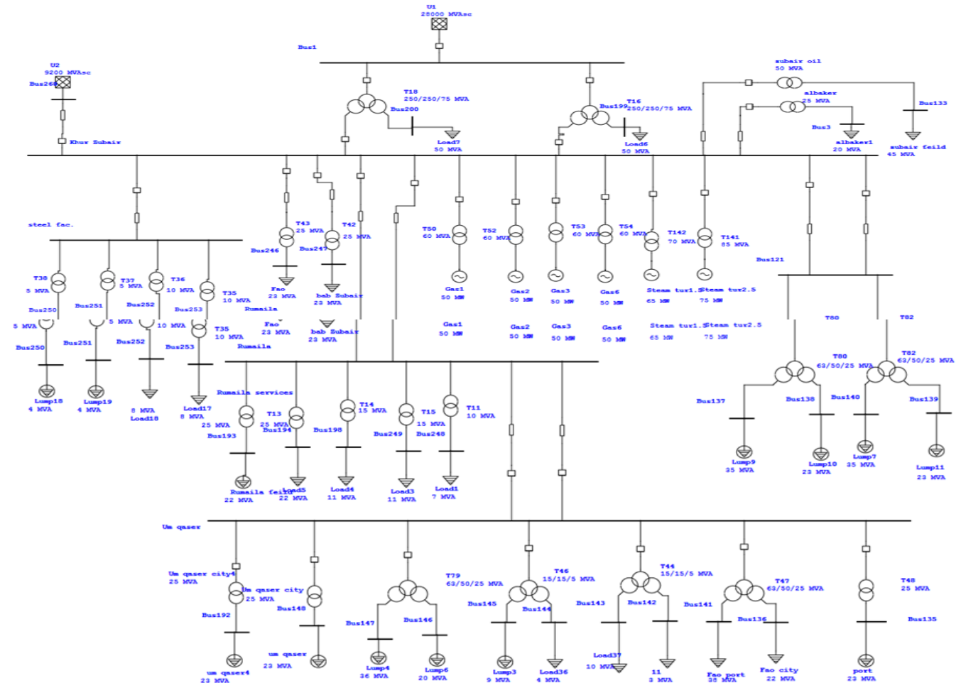
Fig. 1. One-line diagram of 340 MW power plant
