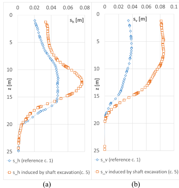
Figure 10. Interaction with an existing tunnel: horizontal (a) and vertical (b) displacements caused by the shaft excavation after tunnelling (case 5) compared to those of the reference case 1 ( d=3\text{m} ).
