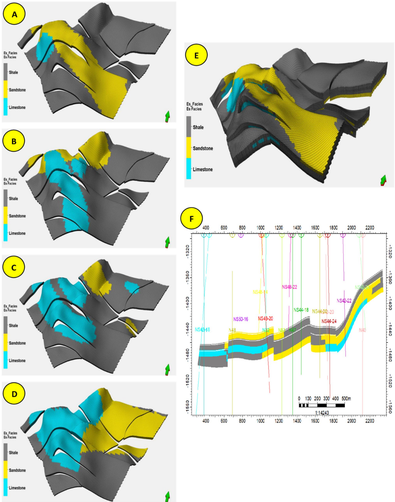
Fig. 9 Facies modeling results for block Nv32. The left panel presents the facies maps of the a. Es1 x 1, b. Es1 x 2, c. Es1 x 3, and d. Es1 x 4 reservoir units. e. Facies modeling of all of the ES1 reservoir units. f. Cross-sectional facies model of the wells used in this study
