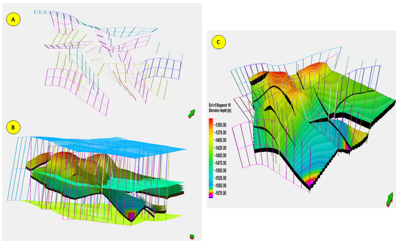
Fig. 4 Structural model of block Nv32. a. Fault pillars and polygons as a structural framework. b. Fault pillars associated with the reservoir horizons. c. Reservoir horizons (Es1 × 1–Es1 × 4), along with the interpreted faults
