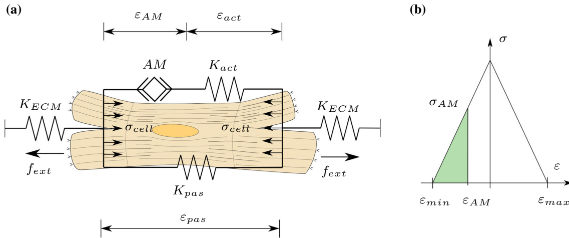
Fig. 2 Cellular mechanosensing model. a Mechanical model of the cell. The contraction of the Actin–Myosin machinery, AM, generates stresses that are transmitted to cell adhesions through the cytoskeleton, which generates active, \varepsilon_{act} , and passive, \varepsilon_{pas} , deformations on the cell elements, as well as the ECM deformation, \varepsilon_{ECM} . \sigma_{cell} represents the stresses resulting from the AM contraction and the resistance to deformation of the active, K_{act} , and passive, K_{pas} , elements, where K_{act} and
