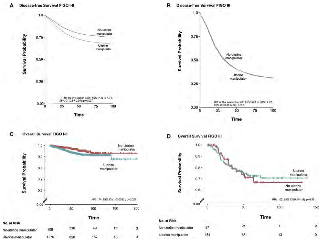
FIGURE 2 Survival analysis
