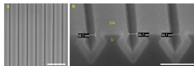
Fig. 5 (a) Top-view (scale bar: 500 nm) and (b) cross-sectional (scale bar: 200 nm) HR-SEM images of a fabricated Si template coated with a SiN layer.
