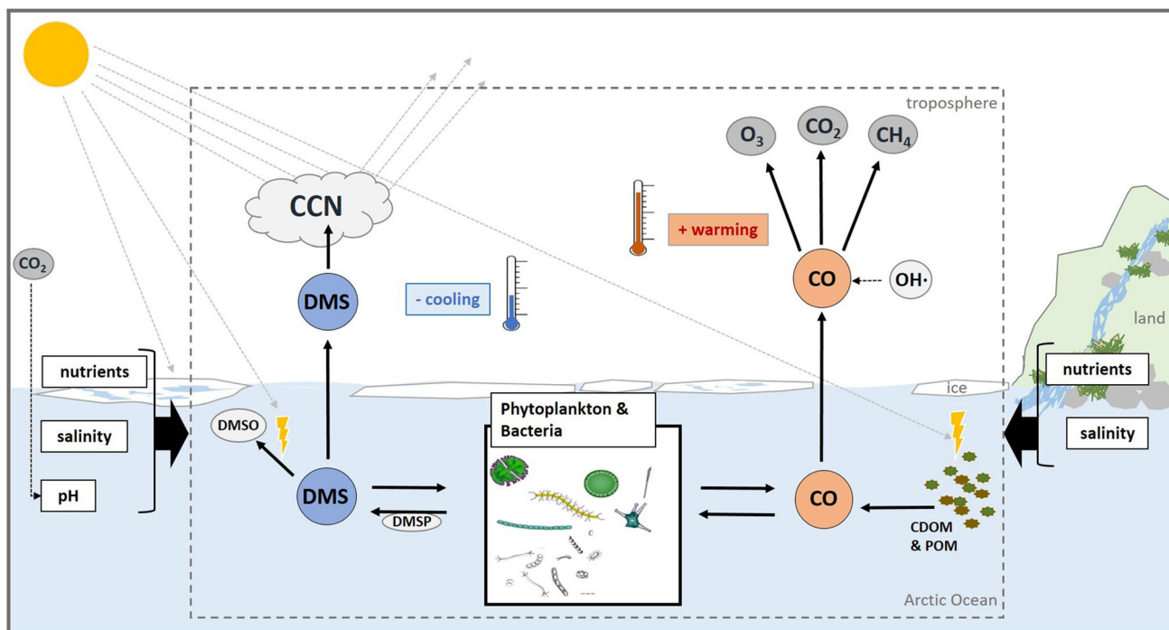
Fig. 1 Schematic view of the interactions of DMS and CO production, consumption and emission pathways in a changing Arctic Ocean. The dashed box marks the processes discussed in this article, comprising interactions in the ocean, ice and atmosphere. Thick arrows outside and towards the box represent changes in nutrients, salinity or pH due to increased ice melt (left side) and/or increased material input from land (right side). Those potentially alter ice-associated and pelagic DMS and CO processes and thus emissions in an uncertain way
