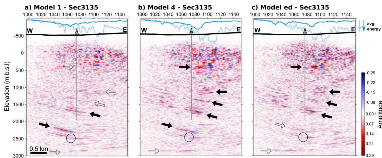
Figure 6. W-E seismic sections (Sec3135) after 3D seismic reflection imaging at the COSC-1 borehole site using three different subsurface anisotropy parameter models and KPSDM. The two solid lines at the top show the average energy of each trace in the upper 1.7 km (light blue) and the depths below (dark blue). The grey line marks the projected position of the COSC-1 borehole location. Arrows mark specific reflections on each section indicating where reflections are differently pronounced (filled: strong; transparent: weak or not visible). The circle highlights a change in the coherence of the reflections. See Figure 1 for the profile location.
