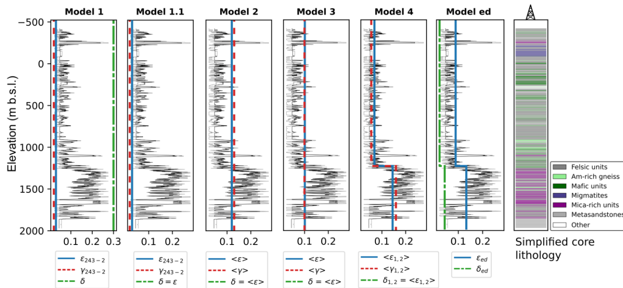
Figure 3. Anisotropy models showing the Thomsen parameters used for the seismic imaging in this study. Model 1: based on Simon et al. (2017); Model 1.1: like model 1 assuming elliptical anisotropy; Model 2: constant parameter model based on the average anisotropy from 16 core samples (Wenning et al. 2016, Kästner et al. 2020a); Model 3: constant parameter model averaged from 1D anisotropy profiles for P- and S-waves indicated by black and grey curves (Kästner et al. 2021); Model 4: two-layer parameter model averaged from 1D anisotropy profile; Model “ed”: variable anisotropy parameter model based on velocity analysis of seismic field data, here shown and averaged at the borehole location for comparison. The simplified core lithology is based on the COSC-1 core description (Lorenz et al. 2015a, b).
