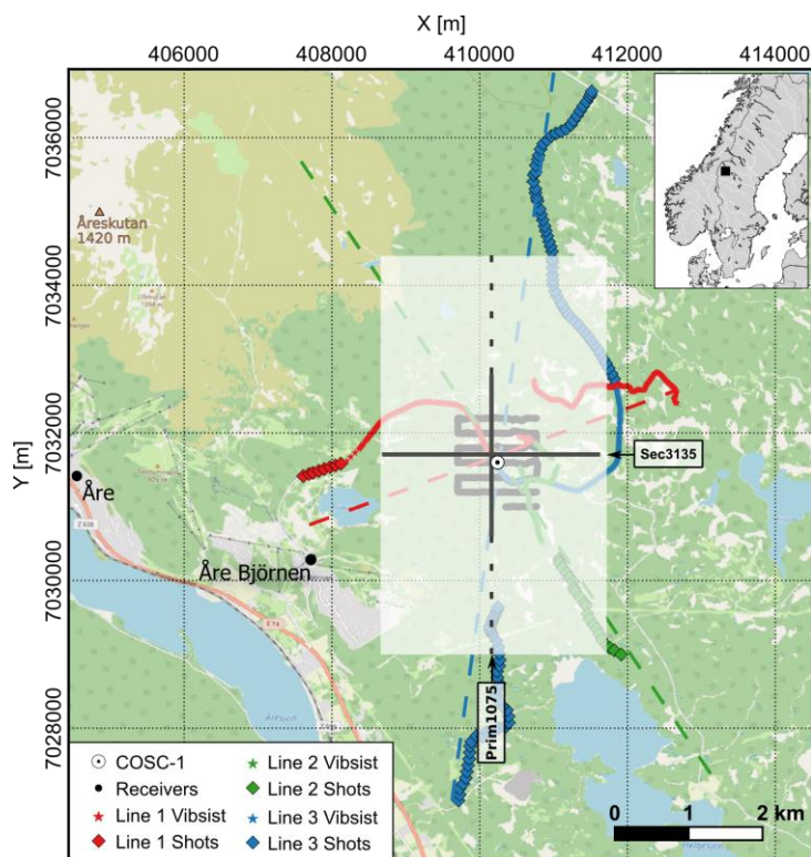
Figure 1. Seismic survey map at the COSC-1 borehole site in Jämtland, Sweden ( 63^{\circ}24'11''\text{N} , 13^{\circ}12'11''\text{E} ; UTM zone 33V). Shown are the 3D seismic reflection survey (Hedin et al. 2016) and the projected 2D tomographic lines (dashed lines; Simon et al. 2017) used for later velocity models. The highlighted rectangle indicates the extent of the CMP grid used in this re-processing.
