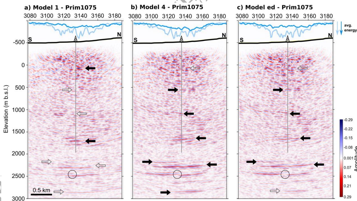
Figure 5. S-N seismic sections (Prim1075) after 3D seismic reflection imaging at the COSC-1 borehole site using three different subsurface anisotropy parameter models and KPSDM. The two solid lines at the top show the average energy of each trace in the
