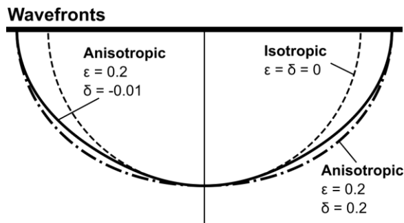
Figure 2. Schematic of seismic wave propagation in a homogeneous anisotropic half space with vertical axis of symmetry showing the angle-dependence of the calculated wavefronts for an isotropic and two anisotropic cases using different values of \epsilon and \delta (adapted from Thomsen 1986).
