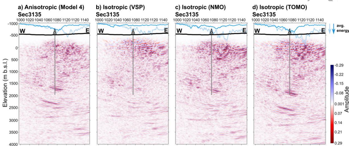
Figure 7. W-E seismic sections (Sec3135) after 3D seismic reflection imaging at the COSC-1 drill site. Seismic migration was applied using an anisotropic velocity model (a) in comparison to isotropic velocity models (b-d) using zero-offset VSP velocities (b), 3D normal moveout velocities (c; NMO), and 2D tomography velocity data (d; TOMO). The two solid lines at the top show the average energy of each trace in the upper 1.7 km (light blue) and the depths below (dark blue). The grey line marks the projected position of the COSC-1 borehole location. See Figure 1 for the location of the section.
