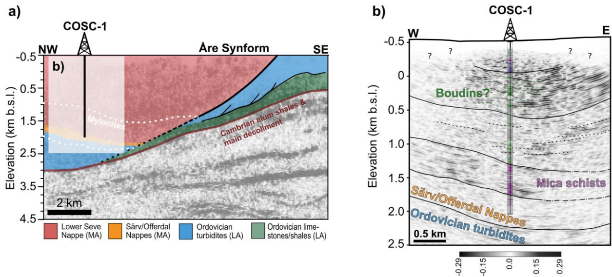
Figure 10. Interpretation of the seismic stratigraphy of the Lower Seve Nappe and underlying tectonic units. (a) Section of the 2D COSC seismic profile interpreted in relation to the tectonostratigraphy of the central Scandinavian Caledonides in western Jämtland, Sweden (Hedin et al. 2012, Juhlin et al. 2016); (b) Re-processed and interpreted 2D seismic section at the COSC-1 borehole site based on limited 3D seismic data (Hedin et al. 2016), here processed and imaged using an anisotropic velocity model from VSP and seismic field data (model ed ). At the borehole location, the lithofacies profile is shown based on the COSC-1 core lithology (modified from Lorenz et al. 2015a).
