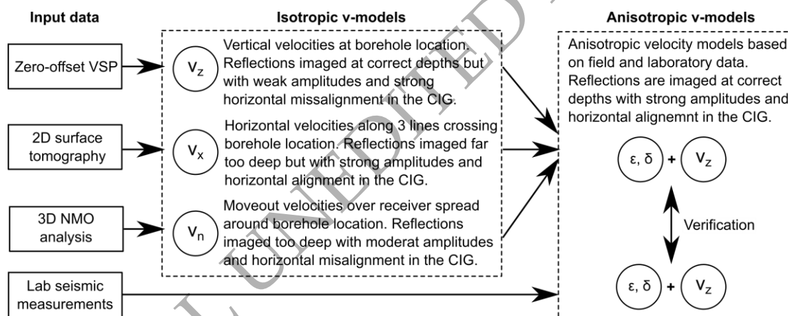
Figure 9. Schematic summarizing the used velocity input data and its effects on the seismic imaging from migrated depth imaging and common image gather at the COSC-1 borehole site.
