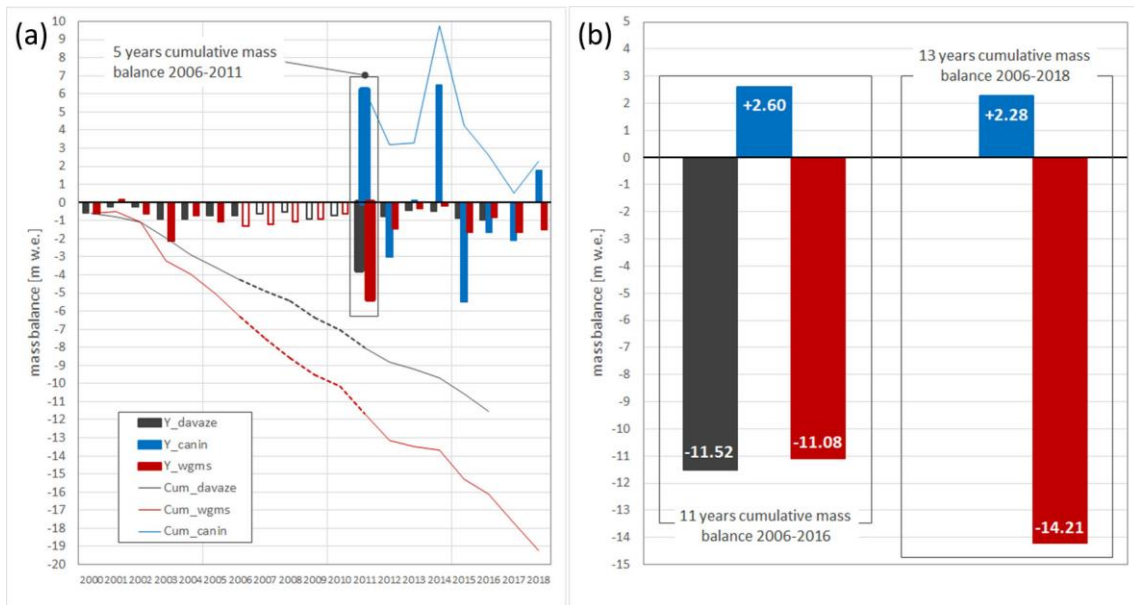
Figure 3. (a) Annual and cumulated geodetic mass balance of the Canin East GIP ( Y_{canin} and Cum_{canin} ) based on a common area (see Figure 2 for details) compared to 2000–2018 WGMS annual and cumulated mass balance in the Alps ( Y_{wgms} and Cum_{wgms} ) and 2000–2016 optical satellite images annual mass balance calculation based on SLA-METHOD [15] ( Y_{davaze} and cum_{davaze} ) [19]; (b) 11 years (left) and 13 years (right) cumulative mass balance for the three records.
