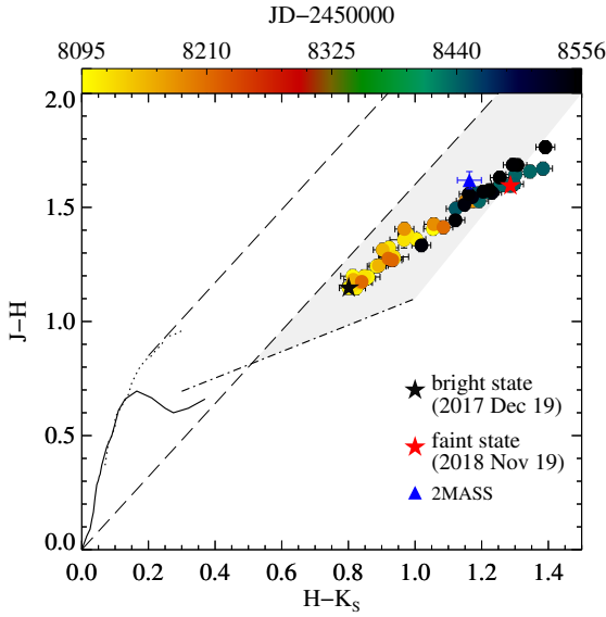
Figure 11. (J-H) vs. (H-K_S) colour-colour diagram. The solid curve shows the colours of the zero-age main sequence, and the dotted line represents the giant branch (Bessell & Brett 1988). The long-dashed lines delimit the area occupied by the reddened normal stars (Cardelli et al. 1989). The dash-dotted line is the locus of unreddened T Tau stars (Meyer et al. 1997) and the gray shaded band borders the area of the reddened K_S -excess stars. The coloured filled circles are SMARTS data, with their colours representing the date of the observations.
