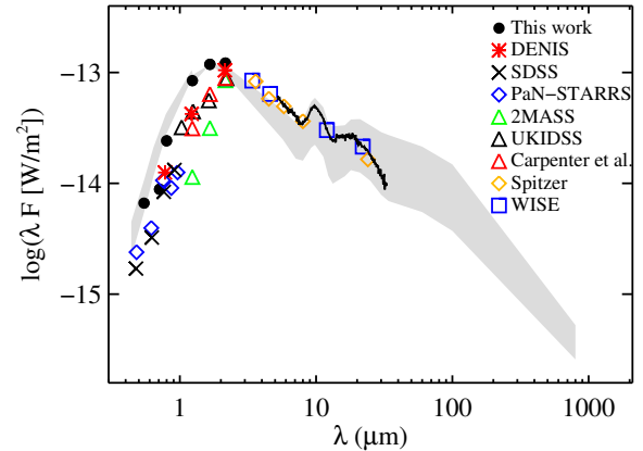
Figure 14. Spectral energy distribution of V555 Ori. The shaded area shows the ‘‘Taurus’’ median SED reddened by the extinction of A_V=2.3 mag determined for the bright state and normalised to the H-band flux measured with SMARTS in the bright state (black circles). The data points below 1.25 \mu\text{m} and above 34 \mu\text{m} are from D’Alessio et al. (1999); otherwise from Furlan et al. (2006). The spectrum, obtained with the Infrared Spectrograph (IRS) of Spitzer was downloaded from the Combined Atlas of Sources with Spitzer IRS Spectra.
