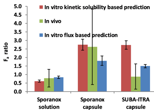
Figure 7. Comparison of the predicted fraction absorbed ratios (fed/ fasted) for the estimation of food effect in the case of Sporanox solution, Sporanox capsules, and SUBA-ITRA capsules and the in vivo data.
