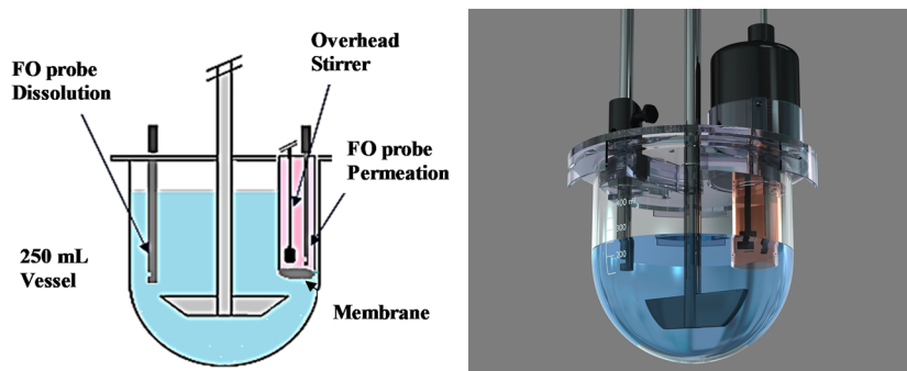
Figure 2. Schematic (on the left) and image (on the right) of the dissolution–flux device used in this study (BioFLUX).
