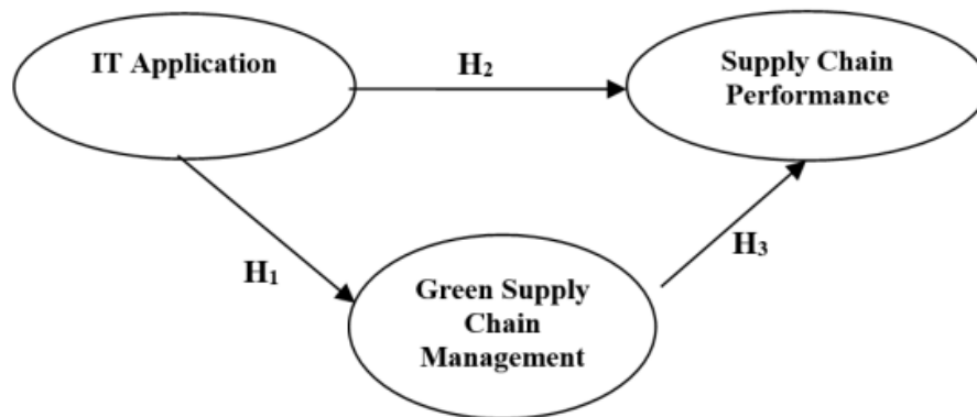
Fig. 1. Research model
