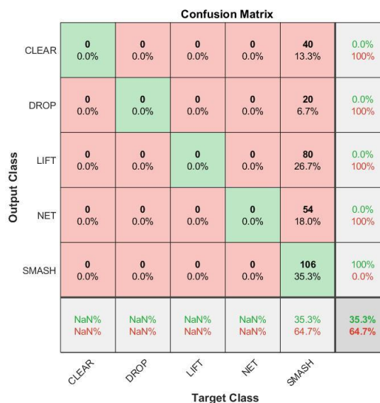
Figure 10. Confusion matrix Vgg-19 Net.
