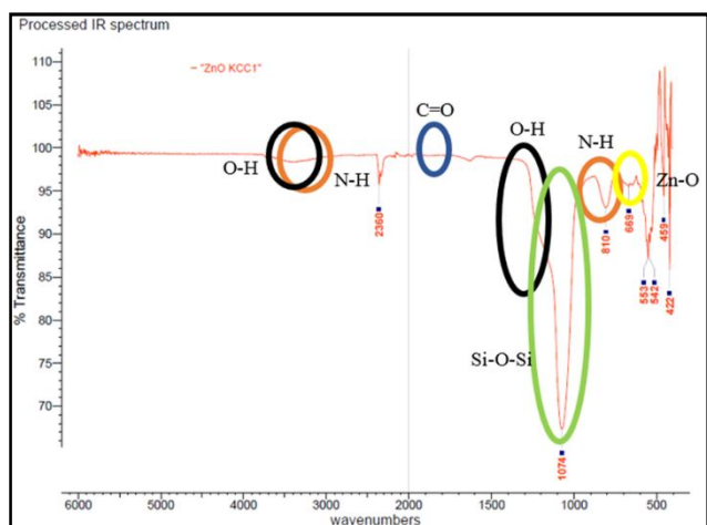
Figure4:FTIR pattern of ZnO-KCC-1
