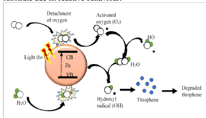
Figure 2: Proposed mechanism illustration for photocatalytic degradation of thiophene
