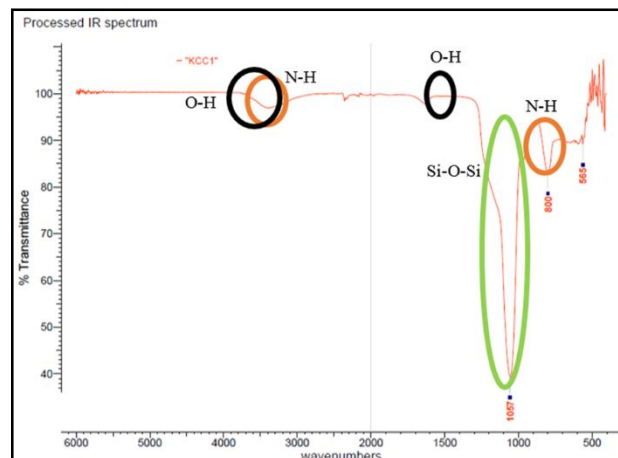
Figure3:FTIR pattern of KCC-1
