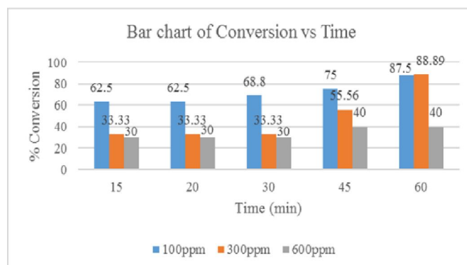
Figure6: Bar chart percentage of conversion against time in minutes.
