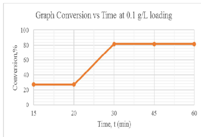
Figure5: Graph of conversion vs time at loading of 0.10 g/L
