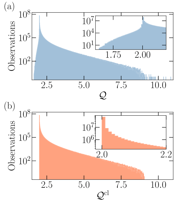
FIG. 3. Histograms of sampled values of (a) Q and (b) Q^{\text{cl}} from Monte Carlo exploration of the parameter space. Insets show the subset of the sampled data in the vicinity of the classical TUR limit. The parameters are sampled from the uniform distributions \gamma_\alpha \in [10^{-4}; 5] , n_\alpha \in [10^{-4}; 10] , \epsilon \in [10^{-4}; 1] , and \Delta \in [0; 1] , and the 10^8 data points are arranged in bins with a width of 0.01.
