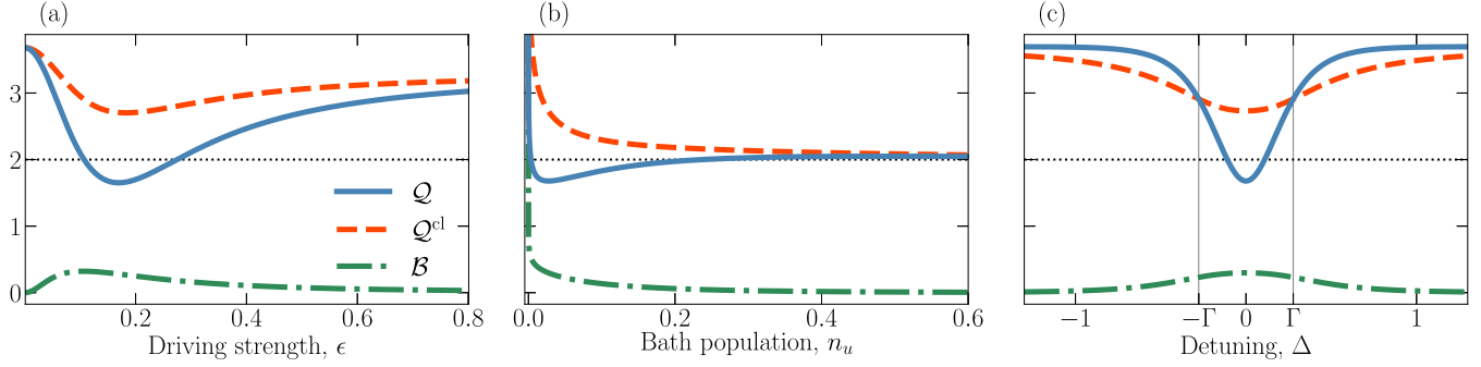
FIG. 2. Probe of thermodynamic uncertainty for the SSDB maser Q (solid blue line) and the classical reference system Q^{\text{cl}} (dashed orange line) along (a) driving strength \epsilon , (b) bath population n_u , and (c) detuning \Delta . The fixed parameters are \gamma_u = 2 , \gamma_l = 0.1 , and n_l = 5 , while the parameters n_u = 0.027 , \epsilon = 0.15 , and \Delta = 0 are varied according to the respective panels. The classical TUR limit is indicated by the dotted black line, and the quantum TUR bound B is indicated by the dash-dotted green line.
