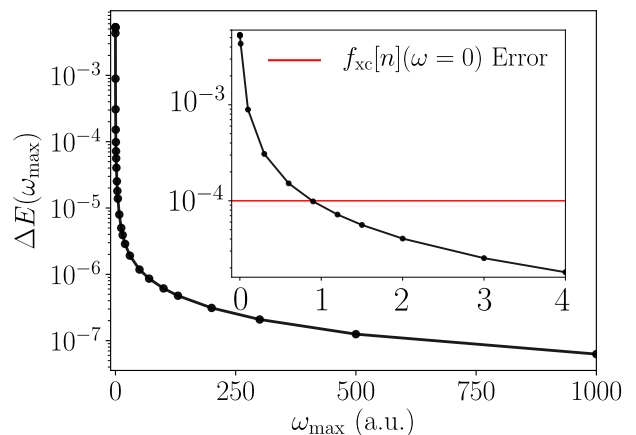
FIG. 8. Absolute error in the slab correlation energy (log scale) with increasing \omega_{\text{max}} (upper bound in the ACFDT \omega -dependent integral). The curve tends toward zero in the \omega_{\text{max}} \rightarrow \infty limit. The inset enlarges the low- \omega region, where it can be seen that the error involved in an AE one-shot ACFDT calculation (red) is contained within 0 < \omega < 1 .
