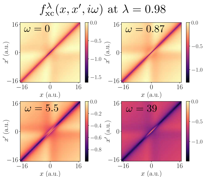
FIG. 9. The exact numerical xc kernel f_{xc}^{\lambda}(x, x', i\omega) for the slab system at \lambda = 0.98 along the adiabatic connection. The xc kernel is depicted at different stages along the i\omega axis, demonstrating that there is little frequency dependence below \omega = 1 a.u., whereupon the xc kernel then deviates from its adiabatic form.
