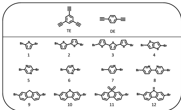
Fig. 1 Structures of the 1,3,5-triethynylbenzene (TE), 1,4-diethynylbenzene (DE) and dibromo-functionalized monomer linkers (1–12) used to synthesize the polymer photocatalysts.
