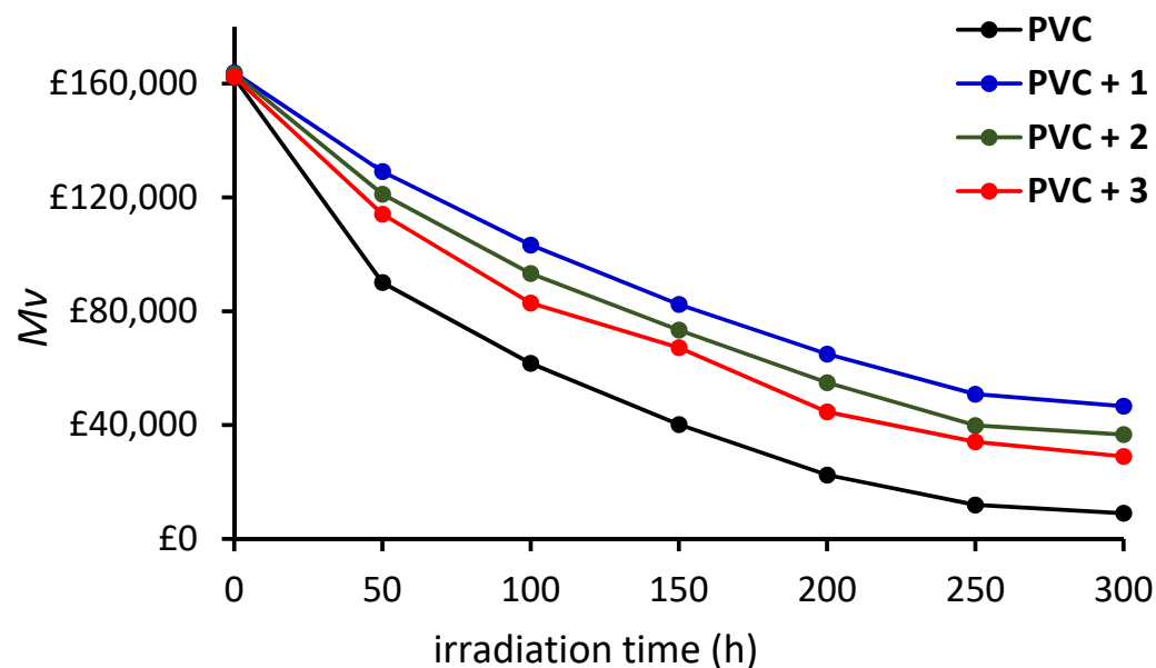
Figure 5. Changes in the \bar{M}_V for PVC films during irradiation.
