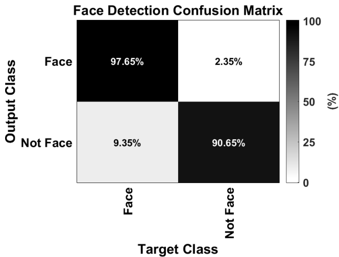
Fig. 5. Confusion matrix showing the percentages of class wise correct vs. incorrect prediction for the face detector.
