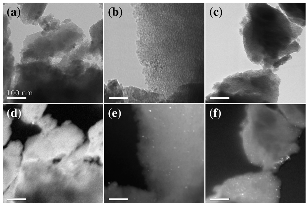
Figure 4. Representative bright field (BF) (a–c) and dark field (DF) (d–f) TEM images of xerogel samples treated at 900 °C with increasing loading of 5 wt% (a,d), 10 wt% (b,e) and 15 wt% (c,f). All scalebars correspond to 100 nm.
