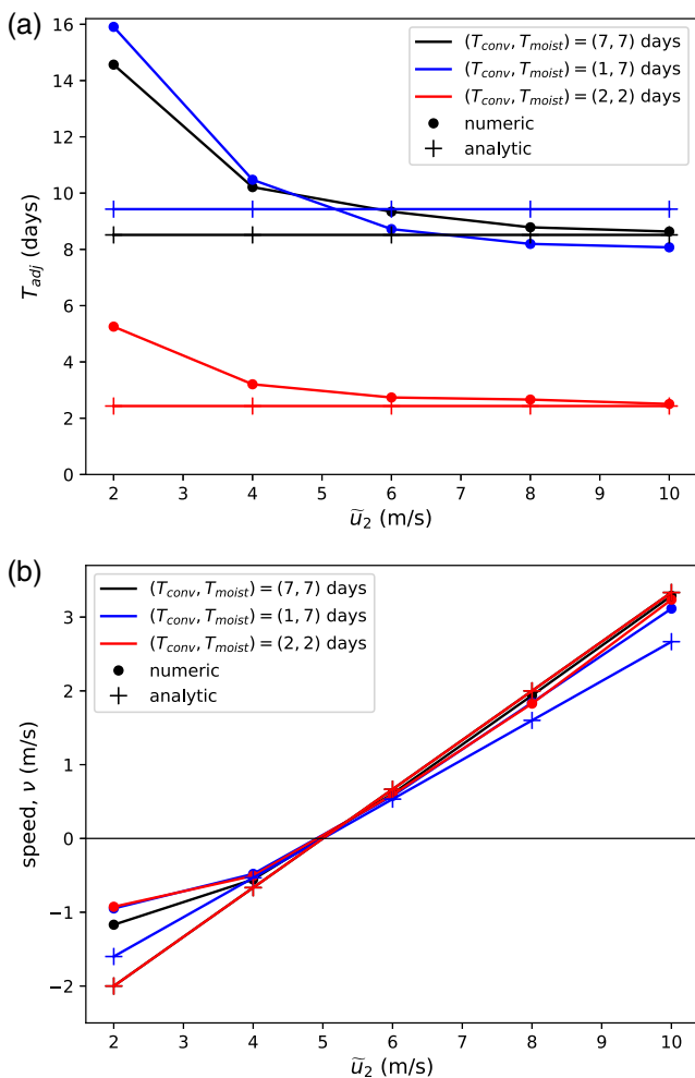
FIGURE 12 Comparing the numerical and analytical derivation of (a) adjustment time, T_{adj} , and (b) onset speed, v , for varying upper-level wind speed, \bar{u}_2 . \Phi = 1 , q_e = 1 , and u_2 = 5 \text{ m}\cdot\text{s}^{-1}
