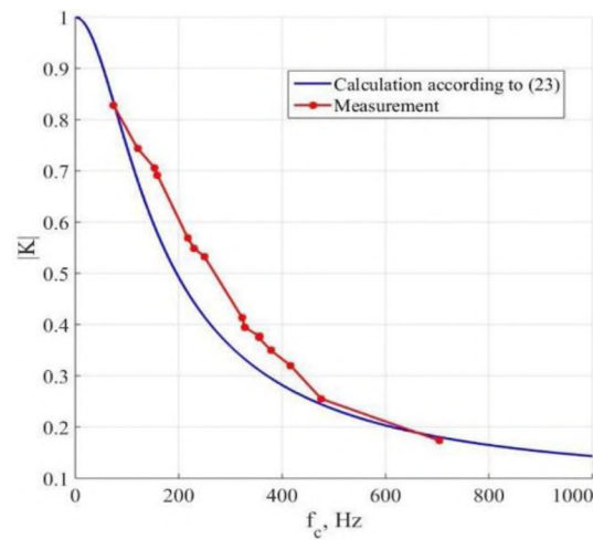
Figure 13. Measured and calculated modulation ratio.
