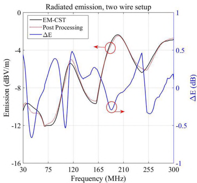
Figure 11. Radiated emission (E field) with ideal termination (2-wire setup).
