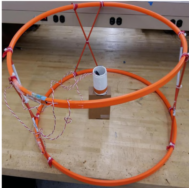
Figure 4. Validation of the receiving coil probe factor using a Helmholtz coil.
