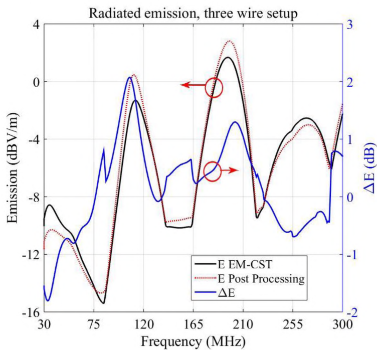
Figure 15. Radiated emission for three-wire setup with TM excitation.
