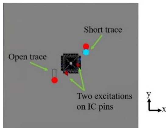
Figure 7. IC with two nearby traces.
