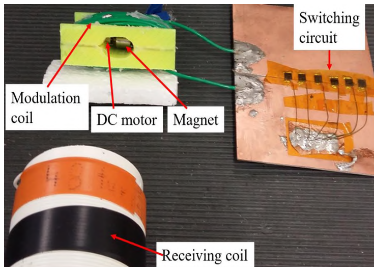
Figure 9. ASK modulation prototype.
