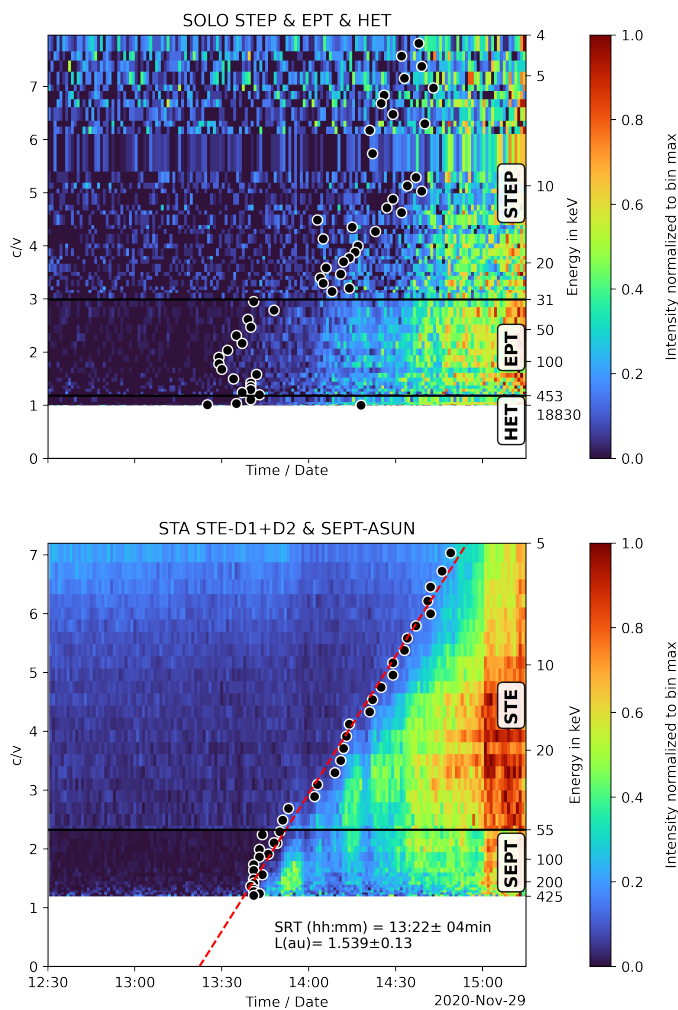
Fig. 6: 60 second time resolution c/v vs. time plots for electrons observed by SoLO STEP, EPT, and HET (top panel) and STEREO STE D1 + D2 and SEPT-ASUN (bottom panel). The color scale represents intensities normalized to maximum intensity in the respective energy channel. Black horizontal lines separate the instruments. Black Points mark the onset times derived with the Possion-CUSUM method. The red dashed line in the bottom panel represents the linear fit for VDA.
