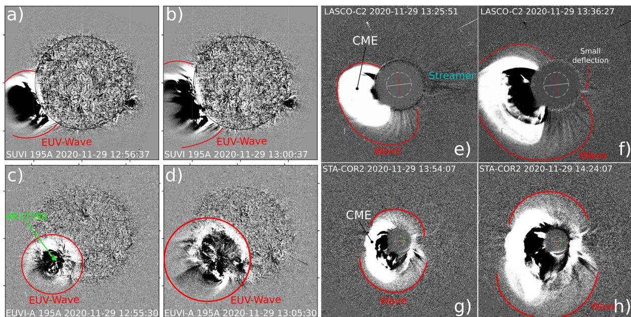
Fig. 3: Remote sensing observations of the EUV wave, the CME, and the white-light shock wave from two different viewpoints. Panels a to d show EUV running-difference images recorded nearly simultaneously from SUVI (a & b) and STEREO-A EUVI (c & d) at 195 Å during the early stages of the EUV wave expansion in the low corona. The EUV wave front is labeled and outlined with the red lines. Panels e to h show running-difference images in white-light from SOHO/LASCO-C2 (e & f) and STEREO-A/COR2 (g & h). The CME is labeled and the white-light shock wave is labeled and outlined with red lines.
