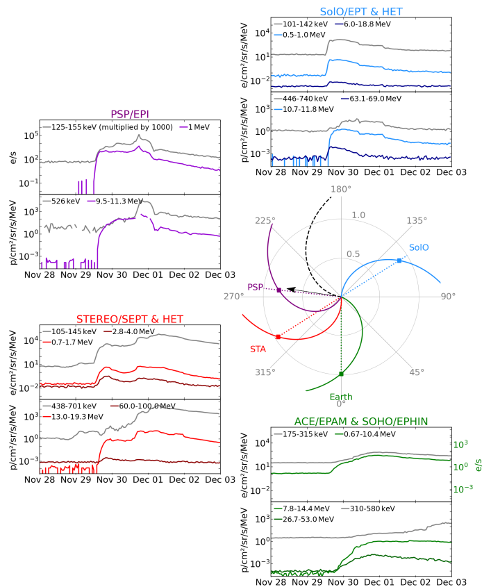
Fig. 1: Overview of the 2020 November 29 SEP event: middle right panel shows the orbital locations of PSP (magenta point), SolO (blue point), STEREO-A (red point), and near-Earth spacecraft (green point) as seen from the north ecliptic. Nominal interplanetary magnetic field (IMF) lines connecting each spacecraft with the Sun considering the solar wind speeds listed in Table 1 are shown in corresponding colors. The black arrow indicates the location of the active region associated with the event (E98 seen from the Earth). Surrounding panels illustrate hourly-averaged proton fluxes (lower panels) and electron fluxes (upper panels) observed by the different spacecraft.
