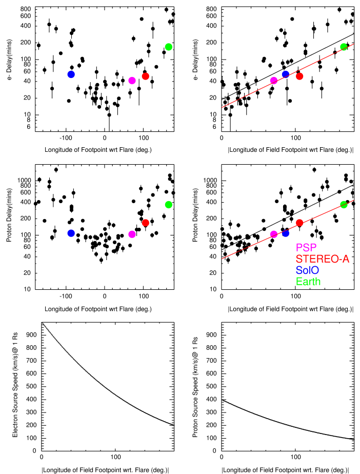
Fig. 10: Comparison of electron (top panels) and proton (middle panels) onset delays vs. connection angle for the November 2020 SEP event (colored circles, indicating the observing spacecraft) with those for \sim 0.7 - 4 MeV electrons and 14 - 24 MeV protons in the cycle 24 SEP events observed at both STEREO spacecraft and near the Earth discussed by Richardson et al. (2014) (black circles). The bottom panels show the “source speeds” from the flare to the field line footpoint as a function of connection angle for electrons (left) and protons inferred from the November 2020 event onset delays.
