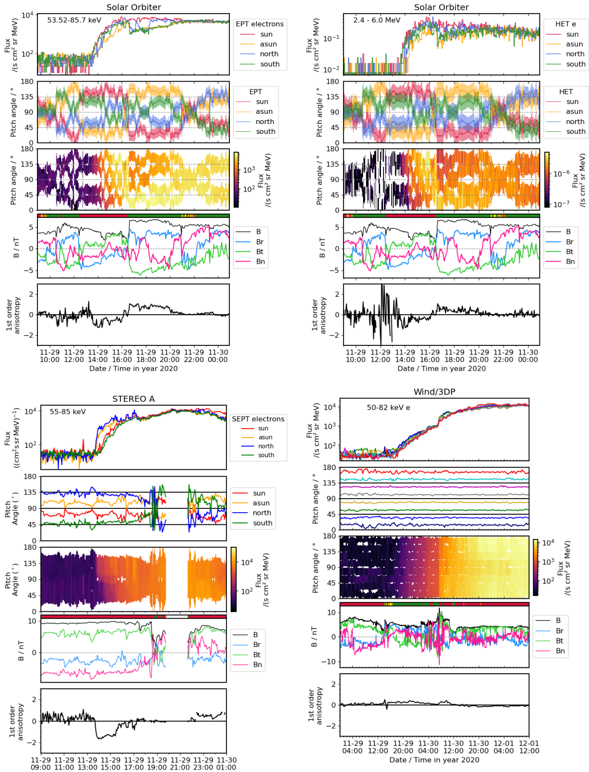
Fig. 8: Pitch angle distributions of energetic electrons observed by SOLO/EPT (top left), SOLO/HET (top right), STEREO A/SEPT (bottom left), and Wind/3DP (bottom right). Top panels show sectorized electron fluxes of \sim 50\text{--}80 keV (bottom figures and top left figure) and 2.4\text{--}6.0 MeV (top right, HET) observed in the four viewing directions of the telescopes (in case of STEREO and SOLO) or binned into eight sectors for Wind. Second panel shows corresponding pitch angles covered by the different viewing directions or sectors, third panel shows pitch angle distributions of the electrons (flux in color coding). The fourth panel shows the magnetic field magnitude and RTN components and the bottom panel shows the first order anisotropy. The colored band on top of the magnetic field panel denotes the in situ magnetic field polarity with red (green) marking negative (positive) polarity and yellow denoting unclear polarity periods. We note the longer time period of the figure showing Wind data.
