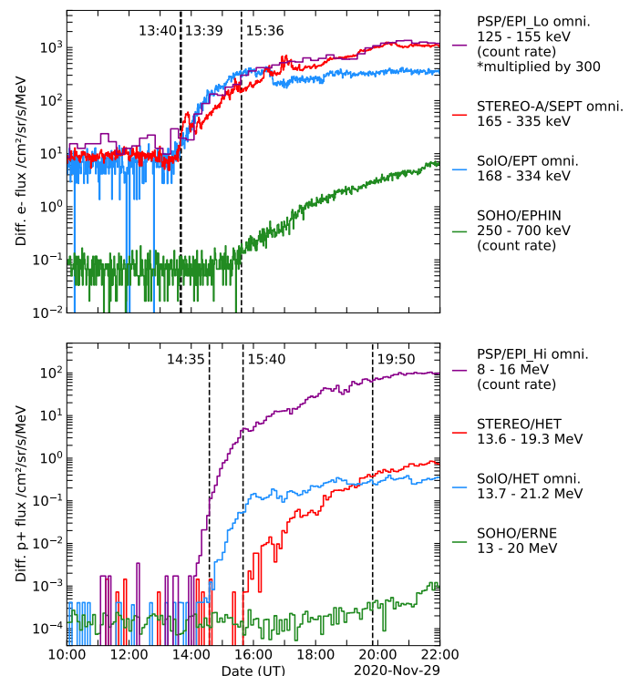
Fig. 7: Electron and proton fluxes observed during the onset phase. Top panel shows 1-minute averaged electron fluxes observed by SoLO/EPT, STEREO-A/SEPT, and SOHO/EPHIN together with 15-minute averaged electron count rates measured by PSP/EPI-Lo. Bottom panel shows 10-minute averaged proton fluxes observed by SoLO/HET, STEREO/HET, SOHO/ERNE and proton count rates measured by PSP/EPI-Hi. 3\sigma onset times are marked by dashed lines.
