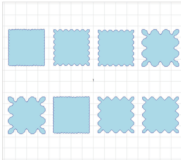
Figure 2: Specimen positions within Fortus 400mc build volume, replication 1
