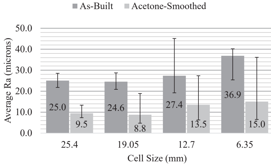
Figure 6: Average surface roughness Ra vs. cell size. The error bars indicate maximum and minimum values
