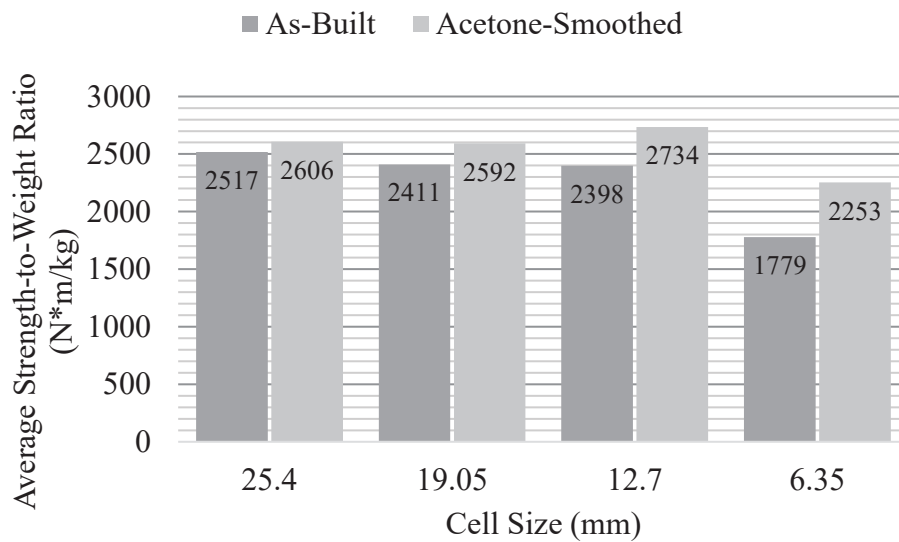
Figure 10: Average strength-to-weight ratio vs. cell size
