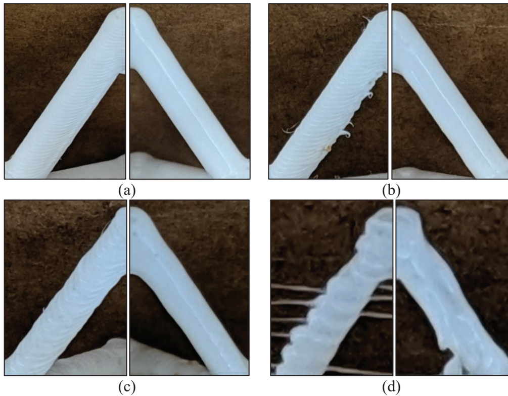
Figure 7: Visual comparison between as-built (left) and acetone-smoothed (right) specimens of (a) 25.40 mm (1.00 in), (b) 19.05 mm (0.75 in), (c) 12.70 mm (0.50 in), and (d) 6.35 mm (0.25 in) cell size
