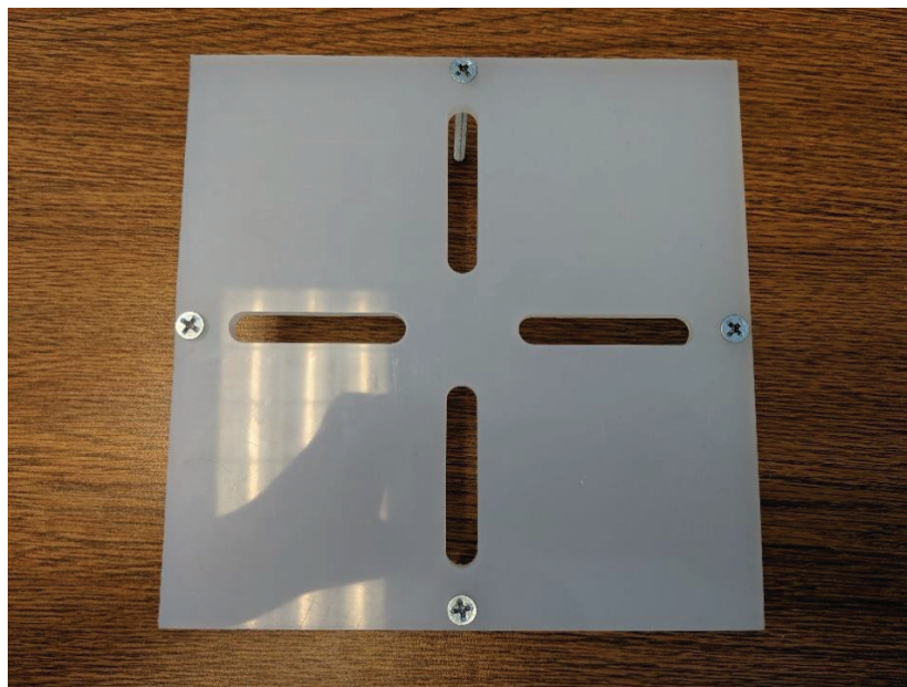
Figure 3: Polypropylene stage for cold acetone smoothing process
