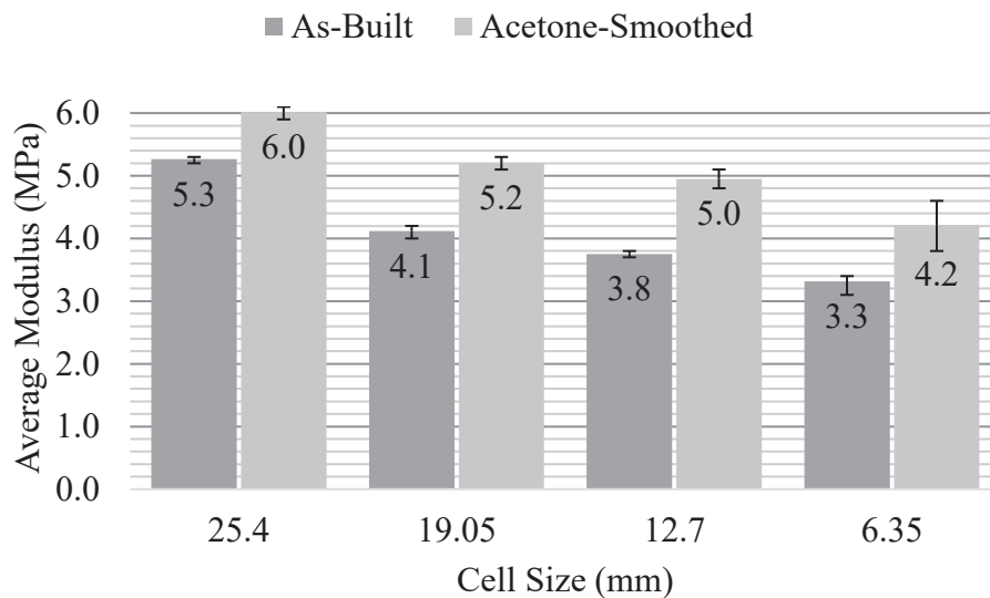
Figure 8: Average elastic modulus vs. cell size. The error bars indicate maximum and minimum values
