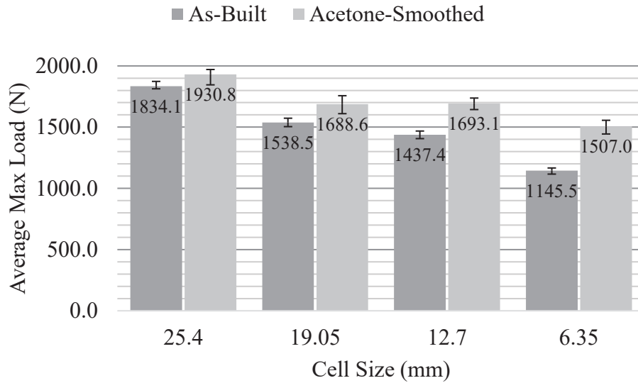
Figure 9: Average maximum load vs. cell size. The error bars indicate maximum and minimum values
