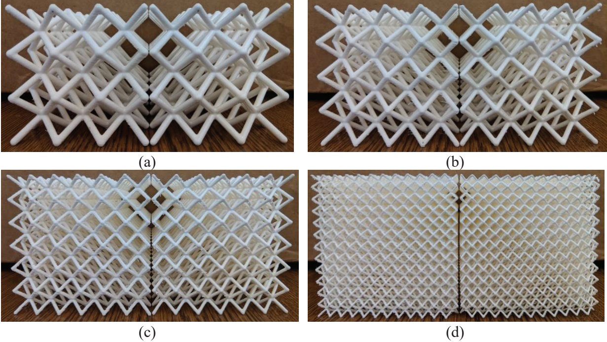
Figure 1: Pictures of one full replication with 8 specimens, with as-built (left) and acetone-smoothed (right) specimens of cell size (a) 25.40mm (1.00 in), (b) 19.05 mm (0.75 in), (c) 12.70 mm (0.50 in), and (d) 6.35 mm (0.25 in)
