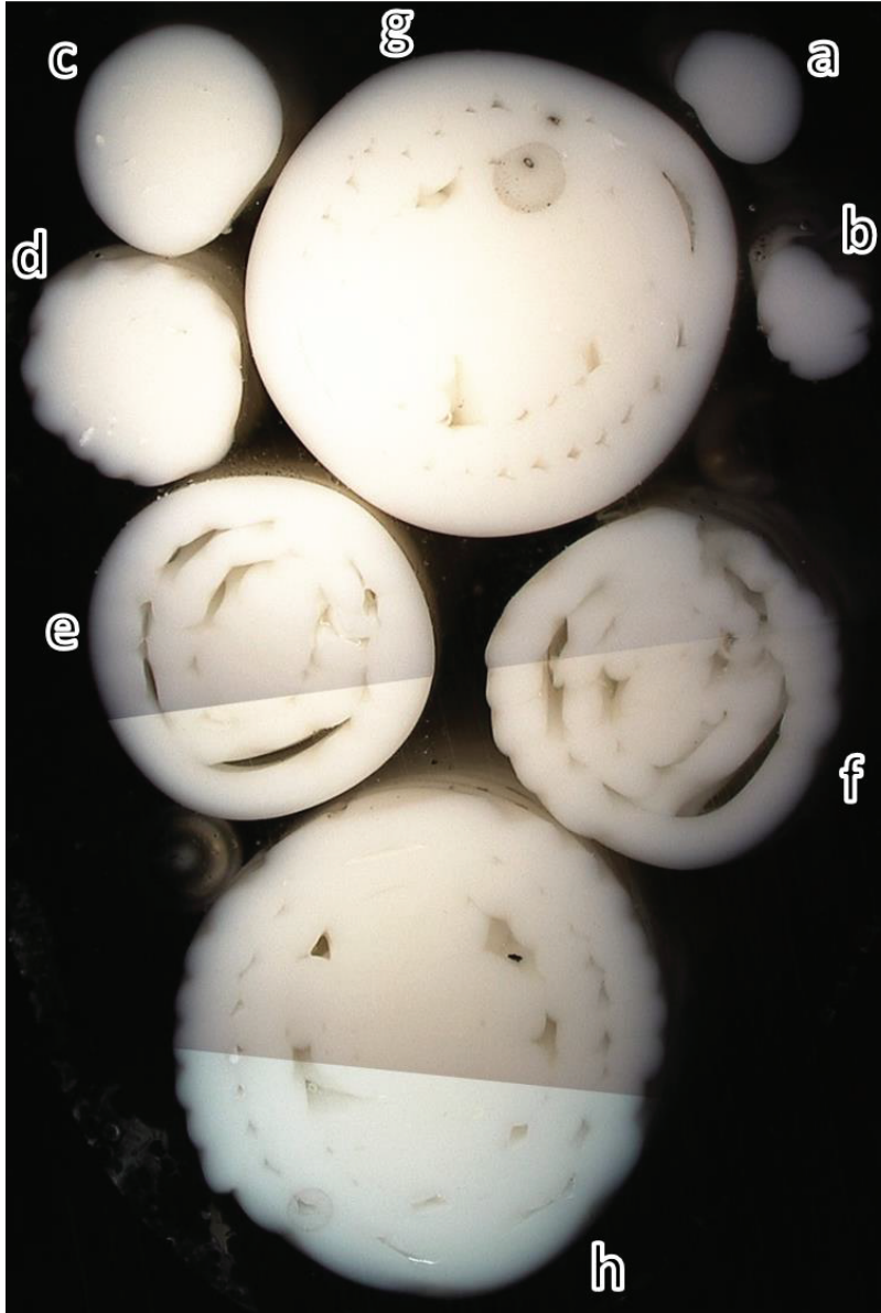
Figure 5: Cross sections of one strut of each treatment combination from replication 1, with (a) acetone-smoothed 6.35 mm (0.25 inch) cell size, (b) as-built 6.35 mm (0.25 inch) cell size, (c) acetone-smoothed 12.70 mm (0.50 inch) cell size, (d) as-built 12.70 mm (0.50 inch) cell size, (e) acetone-smoothed 19.05 mm (0.75 inch) cell size, (f) as-built 19.05 mm (0.75 inch) cell size, (g) acetone-smoothed 25.40 mm (1.00 inch) cell size, (h) as-built 25.40 mm (1.00 inch) cell size
