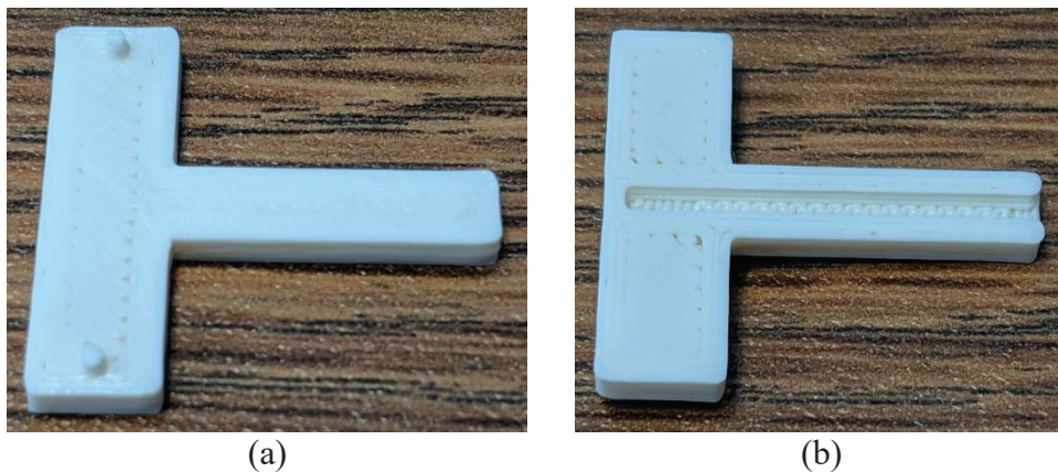
Figure 4: Locating fixture for profilometer measurements: (a) bottom with locating pegs, (b) top with locating groove for lattice structure struts
