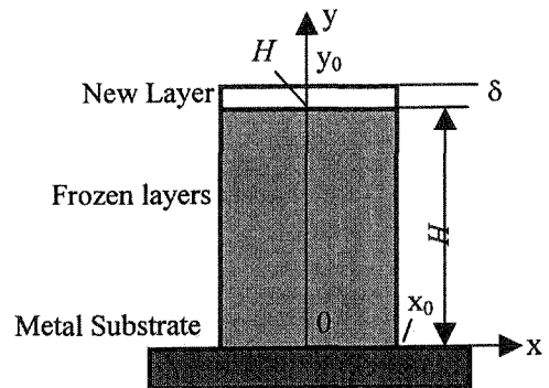
Figure 5. Heat transfer calculation model for Rapid Freeze Prototyping process
