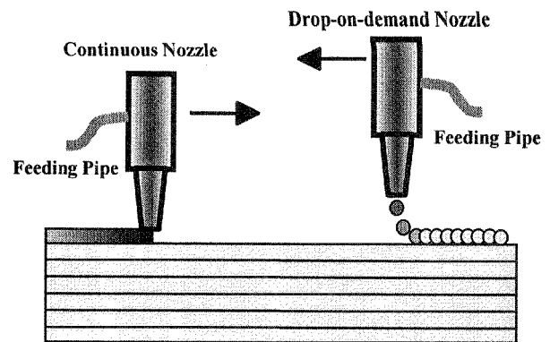
Figure 1. Principles of Rapid Freeze Prototyping
