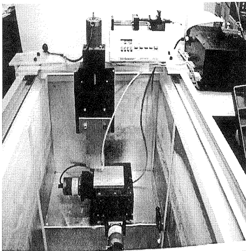
Figure 2. Rapid Freeze Prototyping Experimental Setup
