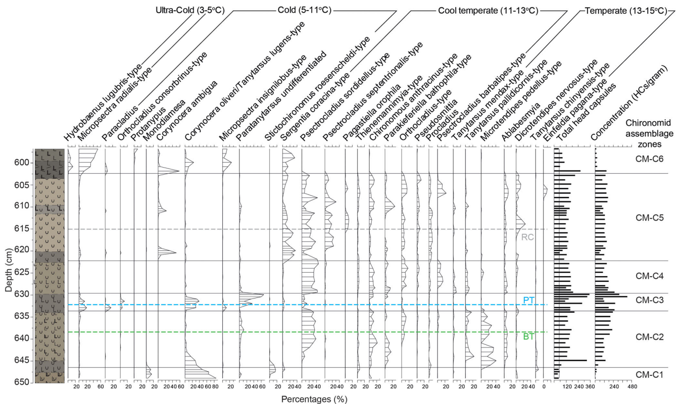
Figure 3. Percentage abundance diagram of selected chironomid taxa present in the Windermere Interstadial (WI) sediments at Crudale Meadow alongside the CRUM1 sequence stratigraphy. The positions of the Borrobol Tephra (BT; 14 107 ± 58 cal a BP) and Penifiler Tephra (PT; 14 024 ± 77 cal a BP) are denoted by the green and blue dashed lines, respectively. The position of the radiocarbon date (RC) is marked by the grey dashed line and has an age of 13 491 ± 67 cal a BP. Chironomid assemblage zones are marked on the right. Taxa are arranged by their T_{optima} in the modern calibration dataset (Heiri et al. , 2011) as calculated using a weighted-averaging model with coolest optima on the left and warmest optima on the right. Head capsule concentrations (HCS/g) and total head capsule counts are displayed on the right. [Color figure can be viewed at wileyonlinelibrary.com]
