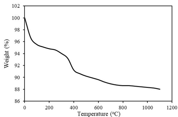
Figure 5. TG analysis of hydroxyapatite
