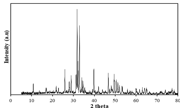
Figure 2. XRD pattern of hydroxyapatite
