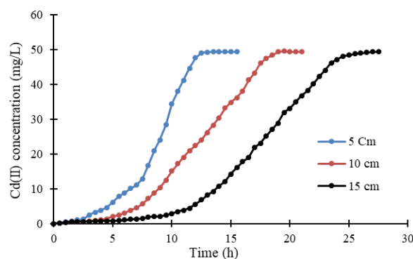
Figure 6. Breakthrough curves for adsorption of Cd(II)
