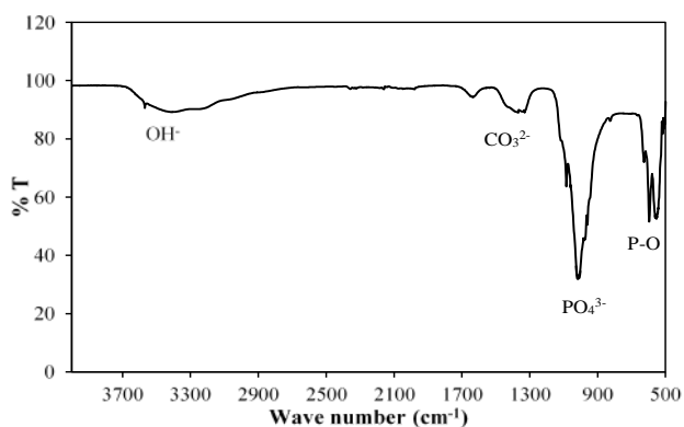
Figure 3. FTIR spectra of hydroxyapatite
