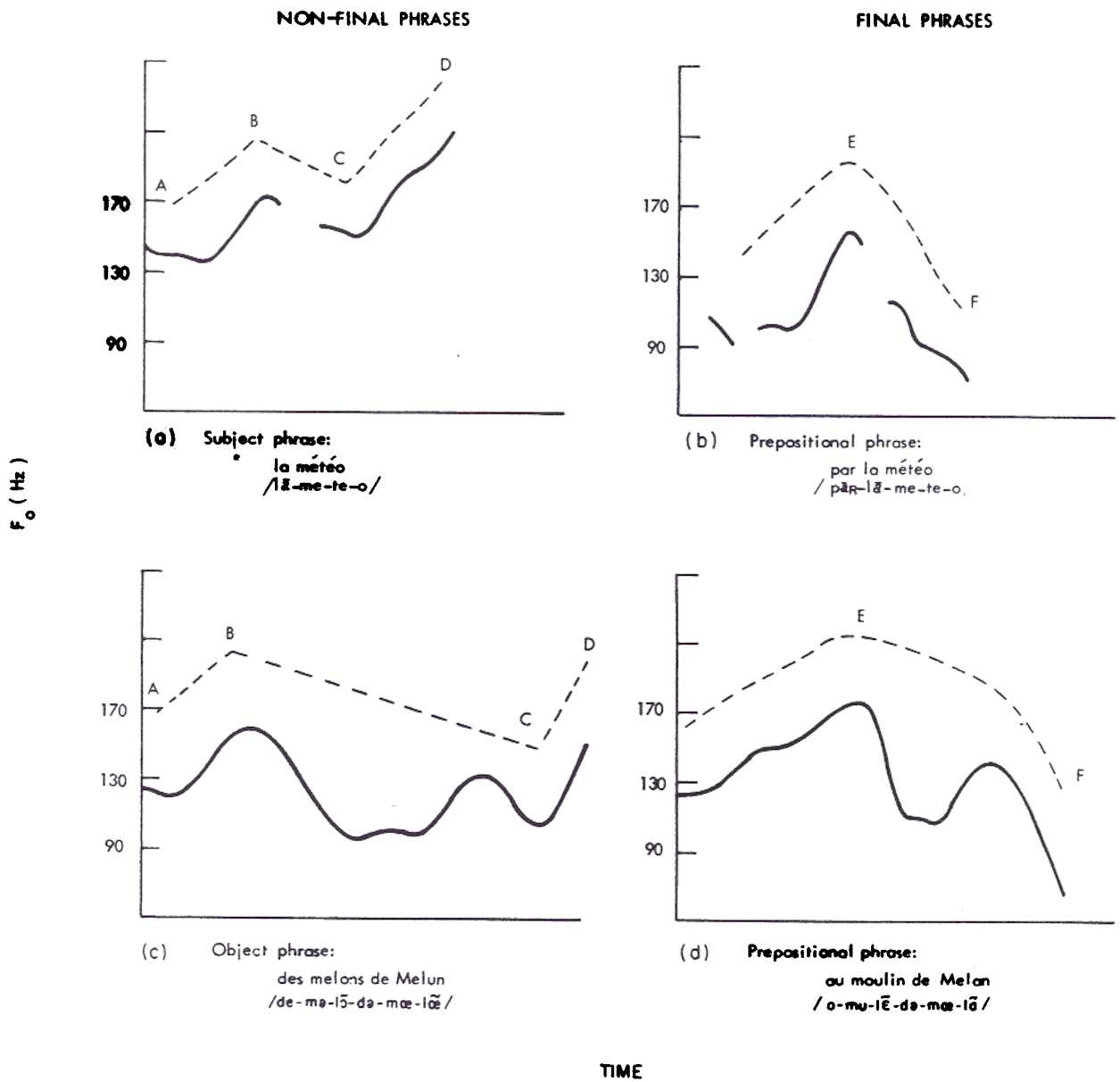
Fig. XVI-22. Typical F_0 patterns for nonfinal phrases and for final phrases. Dashed lines are schematized representations of the contours in which local segmental influences have been ignored.
