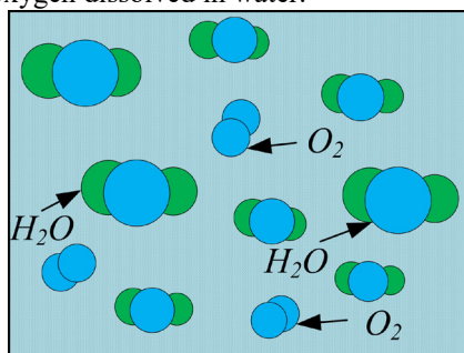
Fig. 1. The O_2 molecules dissolved in water.
