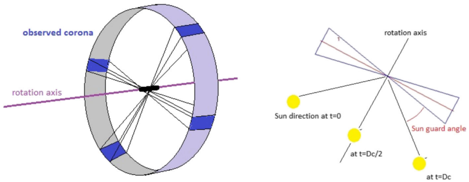
Fig. 1 left: The 22.5 \times 360 \text{ deg}^2 sky corona swept by the instrument every T_s = 2 \text{ min} (rotation period of the platform 8 min). Right: the same corona is observed during D_c , keeping the Sun away by the guard angle (GA).
