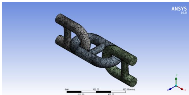
Figure 15. Mesh Element
