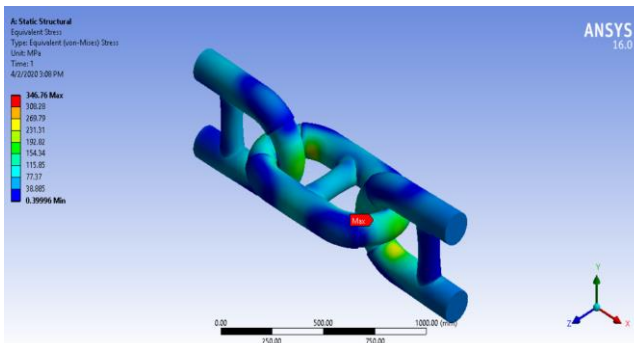
Figure 19. Von Mises Stress in The Third Condition
