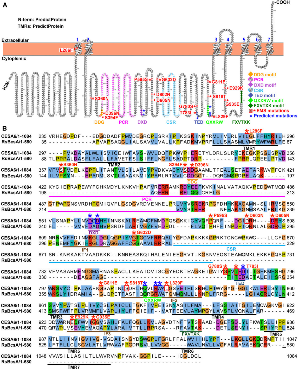
Figure 2. Mutations in CESA6 That Cause Reduced Sensitivity to ES20 Are Mainly Clustered in the Central Cytoplasmic Domain.
