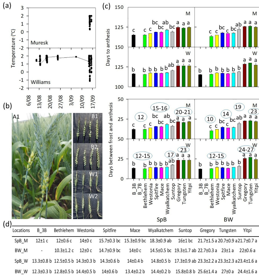
Fig. 1. Frost occurred 9–18 days before anthesis. (a) Daily temperature below 2 °C presented in Muresk and Williams sites (temperature was recorded every 15 min). In Muresk, the low temperature appeared on the 15th and 16th of September 2018 while it mainly occurred on the 14th, 15th, 16th in September, shorter time period on the 11th, 13th, 17th, 18th, 25th of August, and 6th of September in Williams. (b) Different types of frost damage occurred in both Williams and Muresk sites. A1, Frost impacted on the lower part of spikes and the top of peduncles; B1 and B2 showed Bethlehem frost impacted spikes and seed settings, respectively; W1 and W2 showed Westonia frost impacted spikes and seed settings, respectively. (c) Data of days to anthesis and days between last frost event and anthesis on each parental line and control variety in two population areas of SpB and BW in Muresk (M) and Williams (W), respectively. Numbers represent days for different statistical classes. The vertical bars represent SE. (d) Number of days between the frost event and anthesis on different parental lines and control varieties. Empty column means the missing line in the assayed area. Values with the same letter are not different at P = 0.05 .
