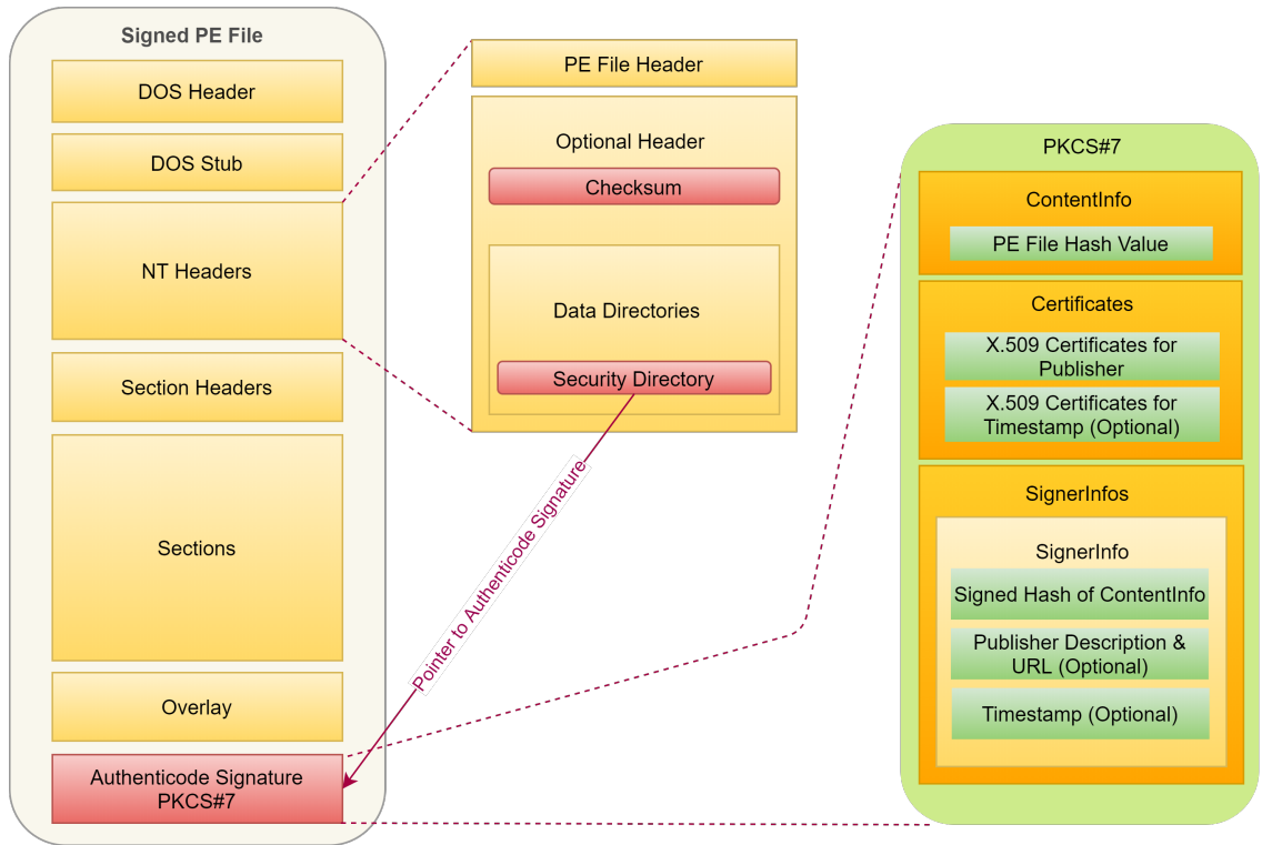
Figure 1: Overview of Signed PE File Format [14].
