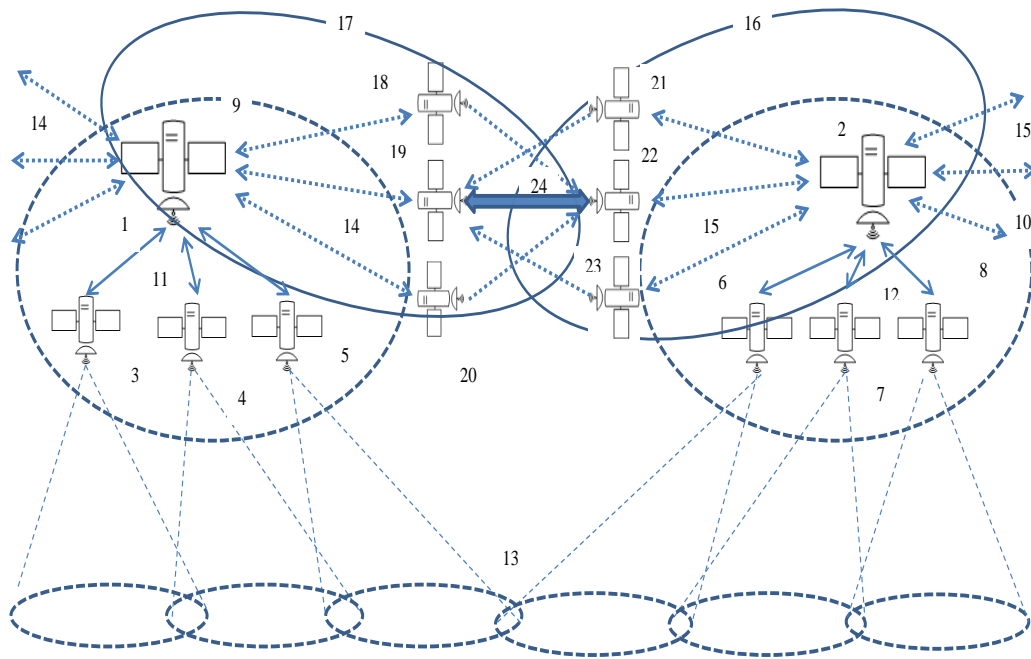
Figure 1: Low-orbit satellite communication system with terahertz communication channels
