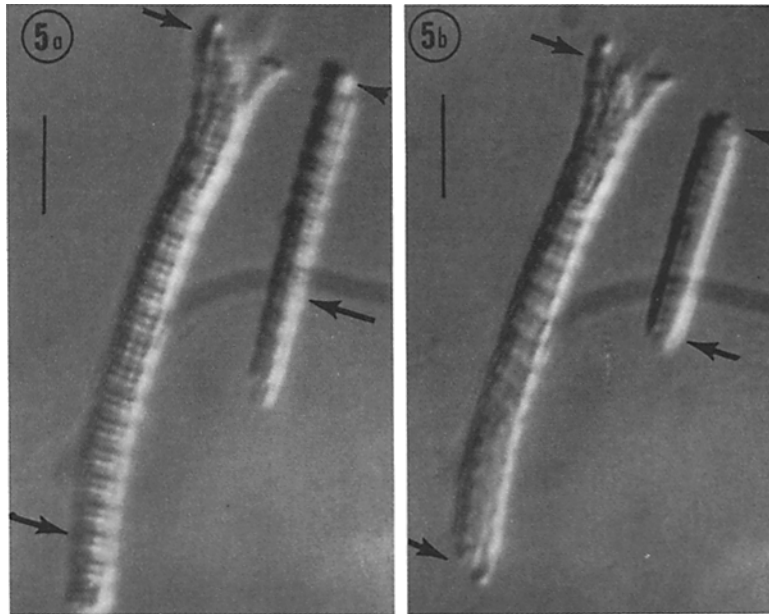
FIGURE 5 Myofibrillar assay of ATP concentration (in this case 1 mM). Nomarski differential interference microscopy. Bar, 10 \mu\text{m} ; \times 1,250. Arrows mark the contracted length. (a) Control. The myofibrils in the absence of added ATP. The sarcomere length for the longer fiber is approx. 3 \mu\text{m} and about 2.7 for the smaller one. (b) Experimental. The myofibrils after the addition of ATP. The sarcomere length is about 2.5 and 1.6 \mu\text{m} for the longer and the shorter fiber, respectively.
