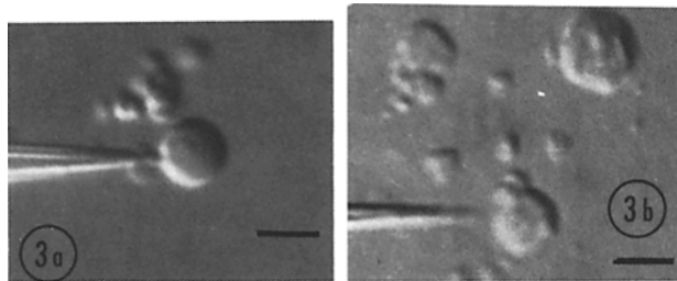
FIGURE 3 Calcium phosphate accumulation in an impaled mitochondrion. The mitochondria are visible with Nomarski differential interference optics. (a) Control. The mitochondrion is impaled in a medium from which \text{CaCl}_2 has been omitted. E = 17 \text{ mV} , R = 1.9 \text{ M}\Omega . Bar, 5 \mu\text{m} ; \times 1,400 . (b) Experimental. A mitochondrion from the same preparation and in the same medium as in (a) is impaled. At zero time 2 \text{ mM CaCl}_2 was added. E = 16 \text{ mV} , R = 2.2 \text{ M}\Omega . Bar, 5 \mu\text{m} ; \times 1,400 .
