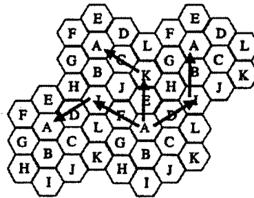
Frequency Reuse Scheme: N = 12
