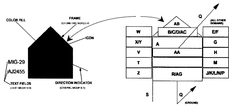
Figure 18. MIL-STD 2525 Symbol Components and Text Field Positions
