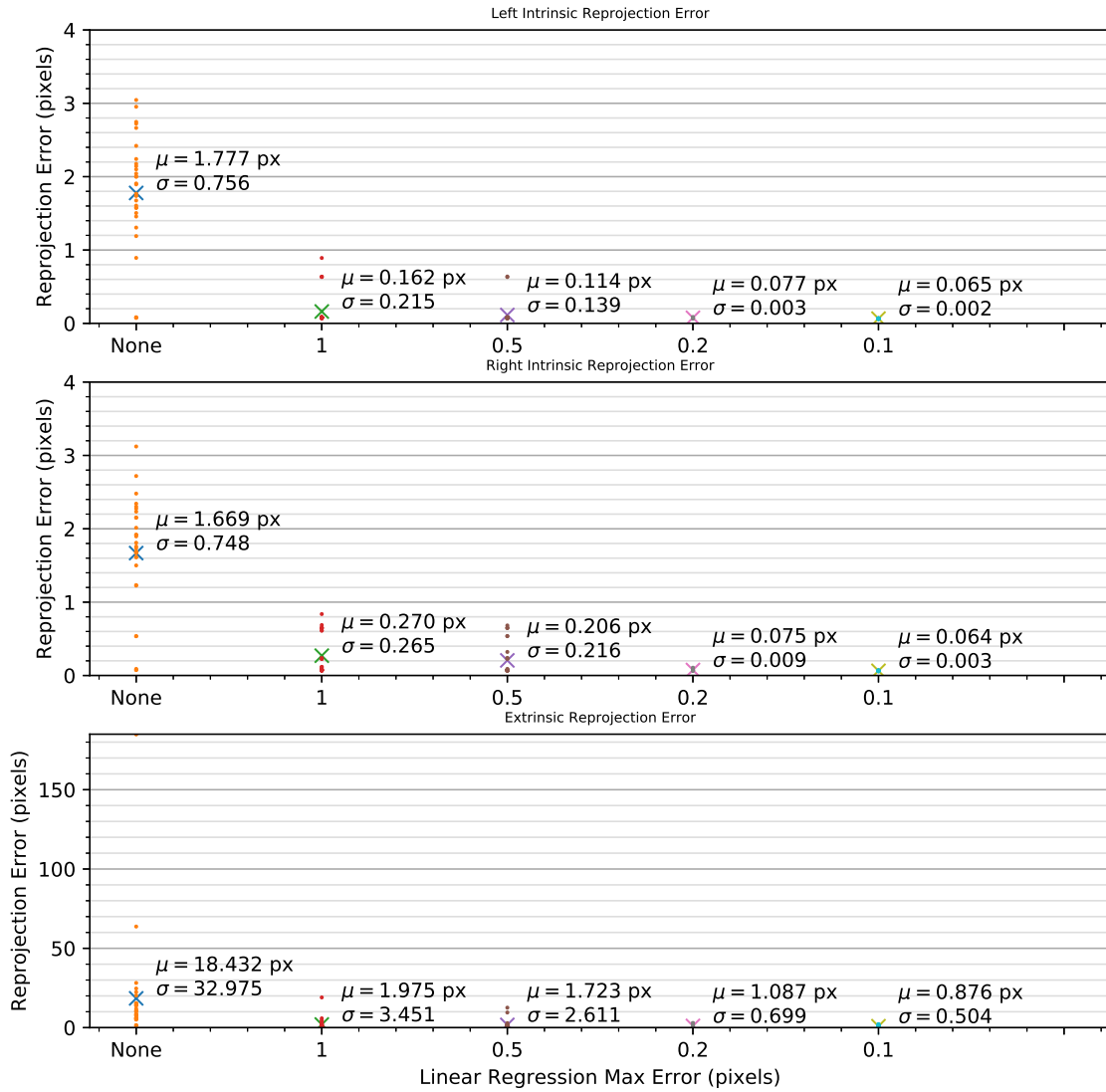
The Effect of Linear Regression Max Error on Calibration Reprojection Error
