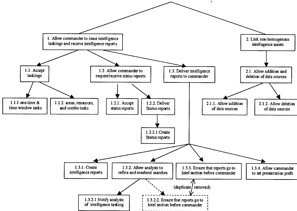
Figure 22: EGADS Goal Hierarchy Diagram
