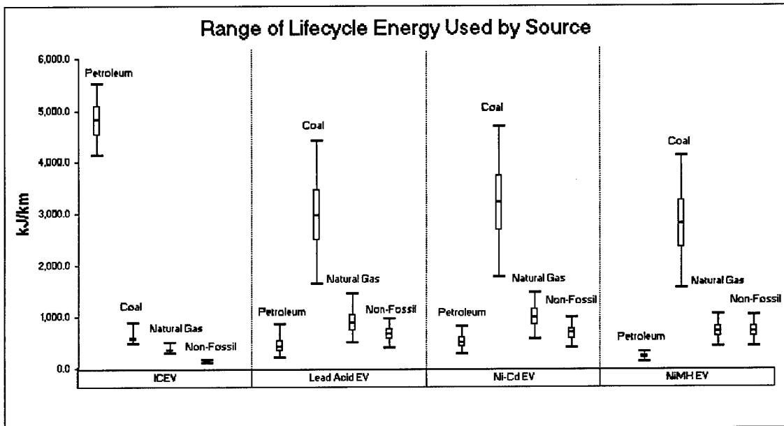
Figure 7. Range of Lifecycle Energy Sources for the Modeled Portion of Vehicle Lifecycle Energy ICEV = Internal Combustion Engine Vehicle EV = Electric Vehicle
