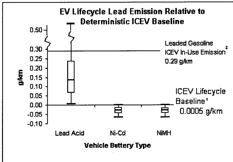
Figure 14. Electric Vehicle (EV) Lifecycle Lead Emissions Relative to Deterministic Internal Combustion Engine Vehicle (ICEV) Baseline 1 Baseline value from Sullivan et al. , 1998 total lifecycle lead emissions divided by a 120,000-mile lifecycle driving distance 2 Historical ICEV lead emissions when lead was an additive in gasoline as predicted by Lave and others 1996
