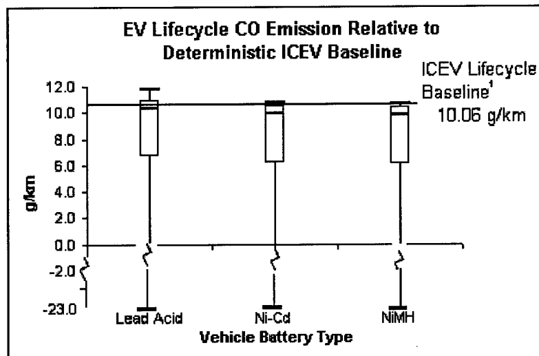
Figure 11. Electric Vehicle (EV) Lifecycle Carbon Monoxide (CO) Emissions Relative to Deterministic Internal Combustion Engine Vehicle (ICEV) Baseline 1 Baseline value from Sullivan et al. , 1998 total lifecycle CO emissions divided by a 120,000-mile lifecycle driving distance
