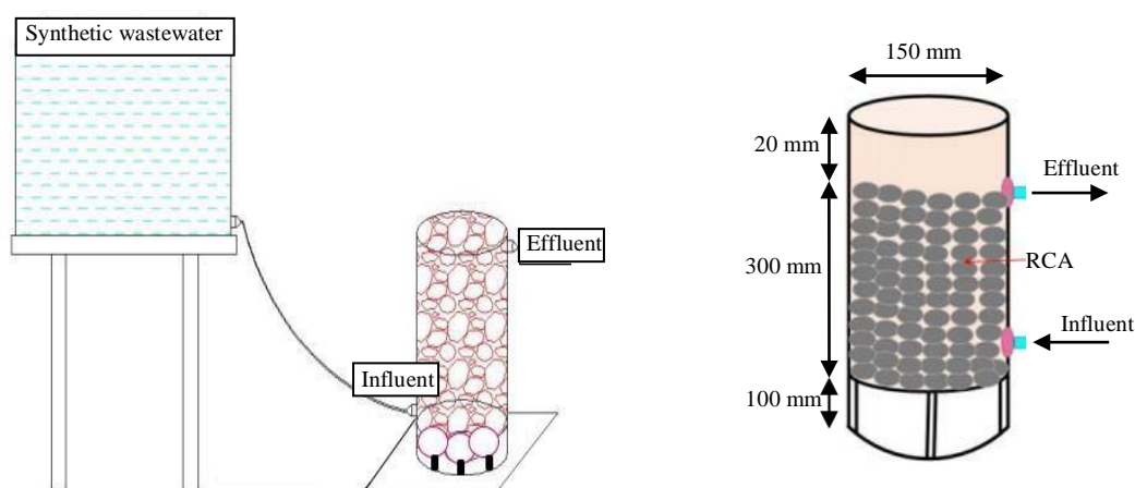
Fig. 2 - The schematic diagram for filter arrangement Fig. 3 - The dimension of the lab-scale column filter
