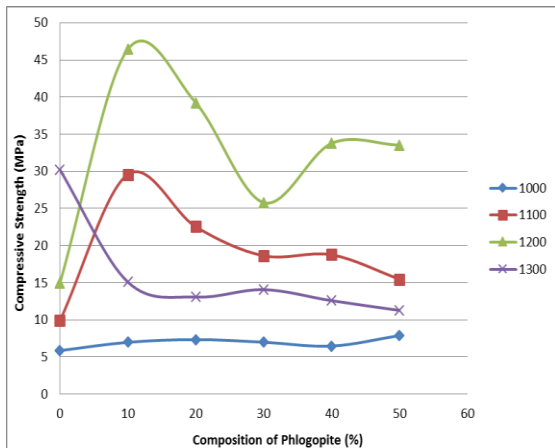
Figure 3 Graph of the compressive strength of porcelain against composition of phlogopite at different sintering temperatures.
