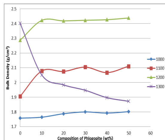
Figure 2 Graph of the bulk density of porcelain against composition of phlogopite at different sintering temperatures
