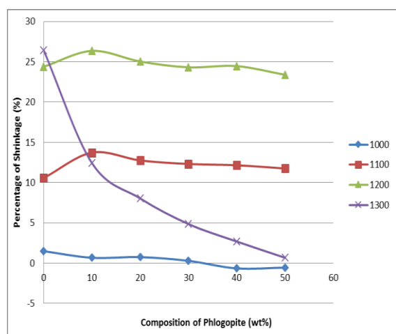
Figure 1 Graph of the percentage of porcelain shrinkage against composition of phlogopite at different sintering temperatures
