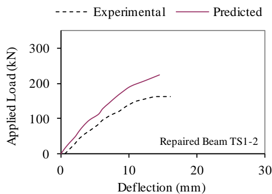
(b) CFF repaired beam TS1-1
