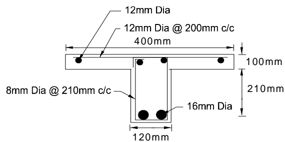
(b) Cross-section
